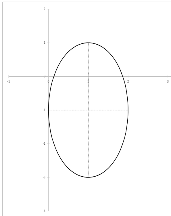
Figure 13: Ellipse with [h, k, a, b, v] = [1, -1, 1, 2, 2]
