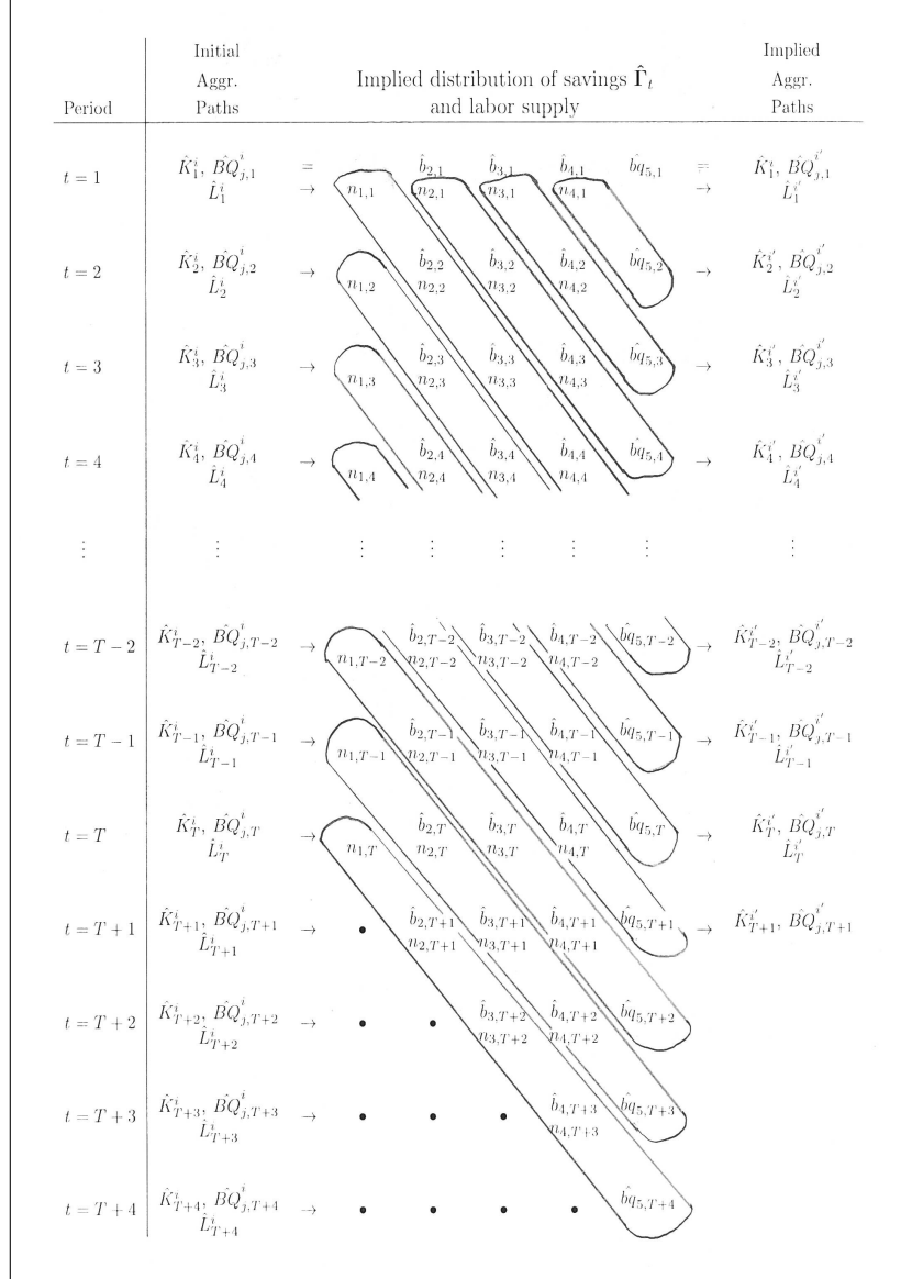
Figure 16: Diagram of TPI solution method within each iteration for S = 4 and J = 1
