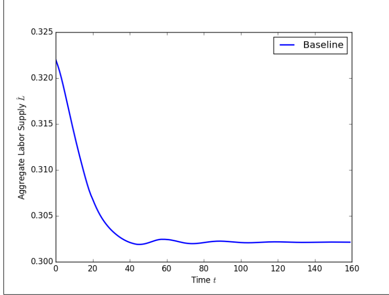
Figure 15: Equilibrium time path of L_t for S = 80 and J = 7 in baseline model
