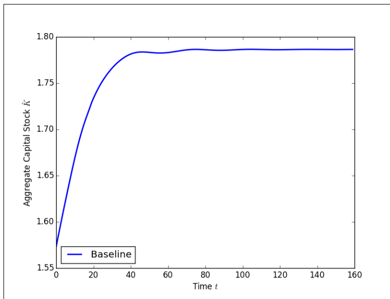
Figure 14: Equilibrium time path of K_t for S = 80 and J = 7 in baseline model
