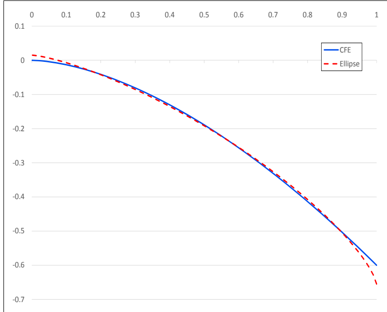
Figure 12: Comparison of standard utility of labor n to elliptical utility
