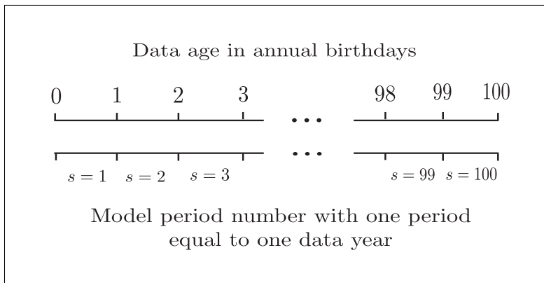
Figure 5: Correspondence of model timing to data timing for model periods of one year
