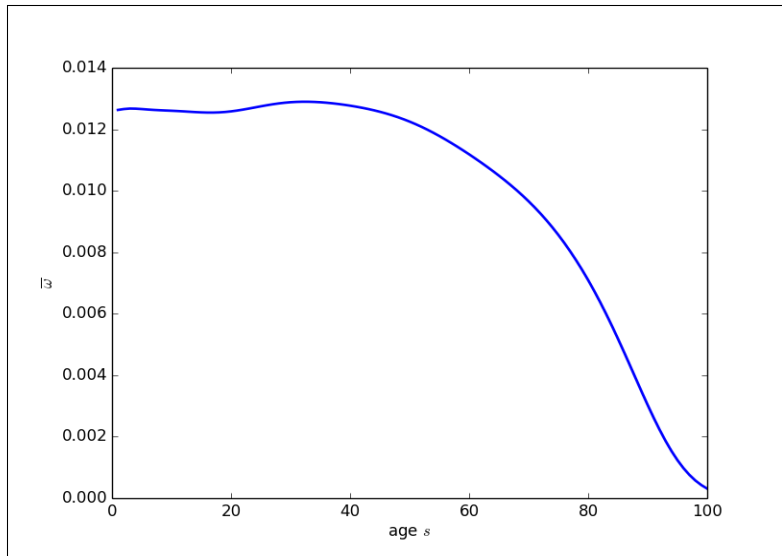
Figure 11: Steady-state population percent distribution by age \bar{\omega}
