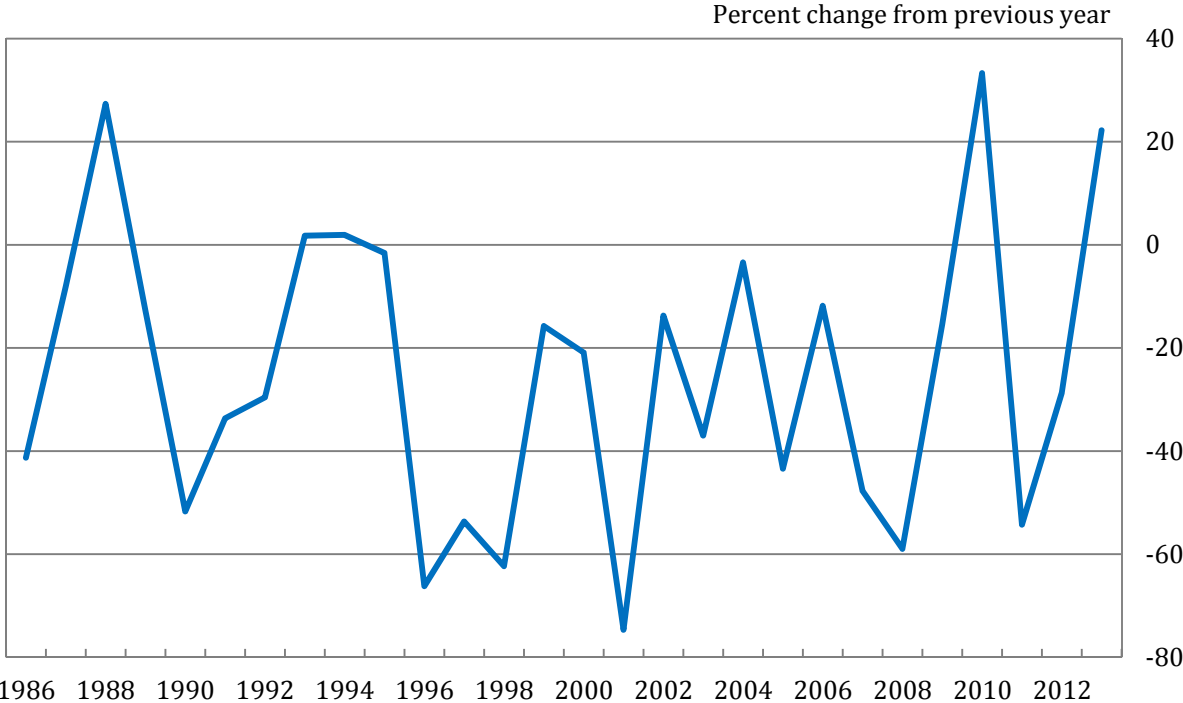
Figure 3: DRAM Prices
