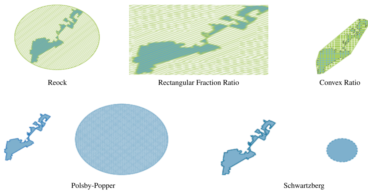
Figure A.4. Examples of Compactness Measures
