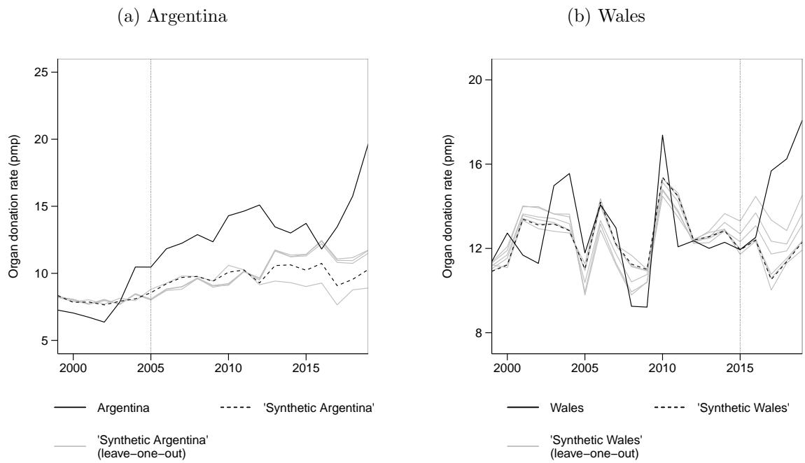
Figure 6: Leave-one-out procedure
