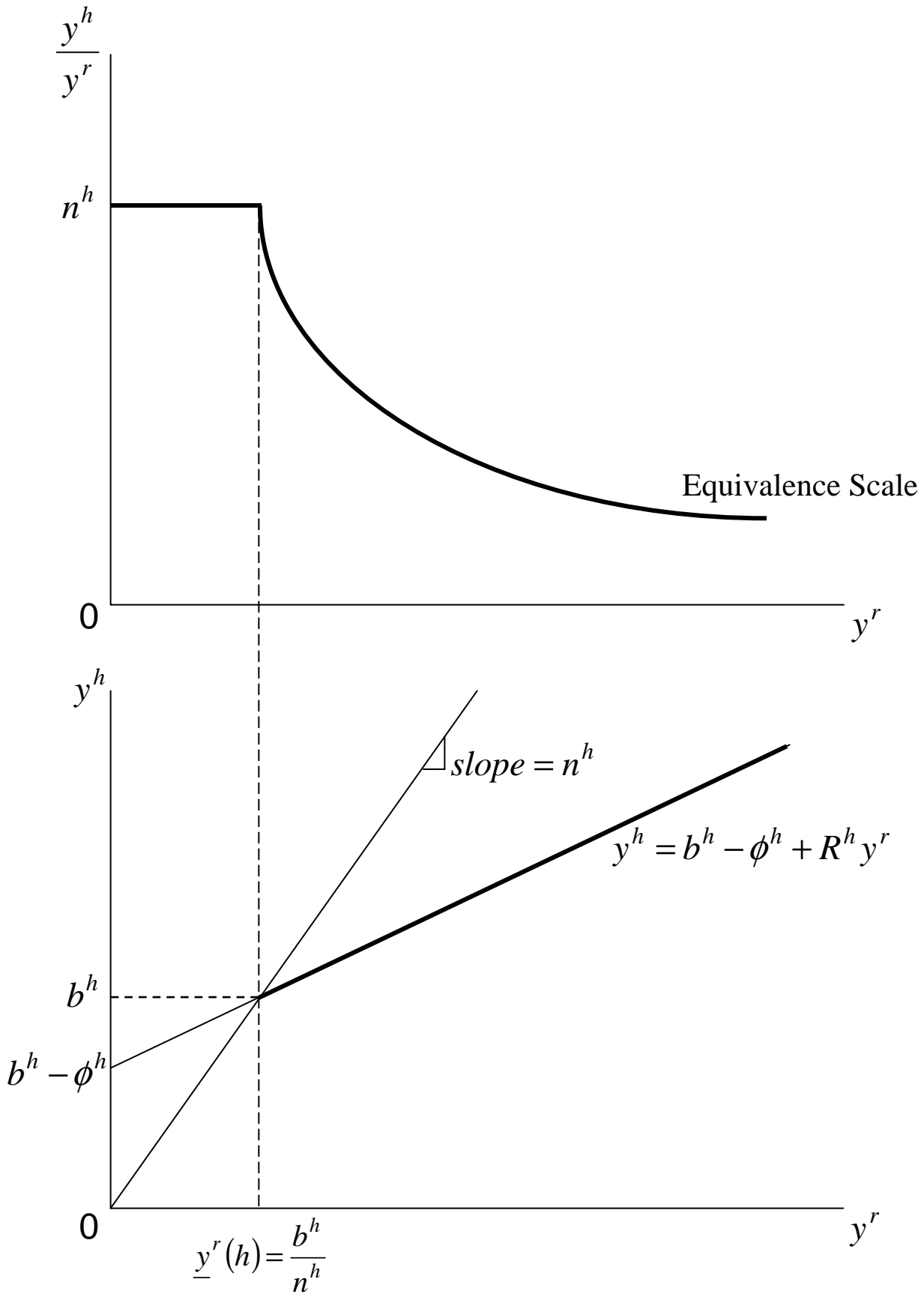
Figure 1 Identification of the family-type subsistence level, b^h
