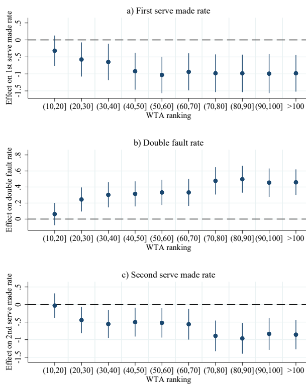
Figure A.1: Relation between ATP/WTA ranking and tennis performance with player and opponent FE
