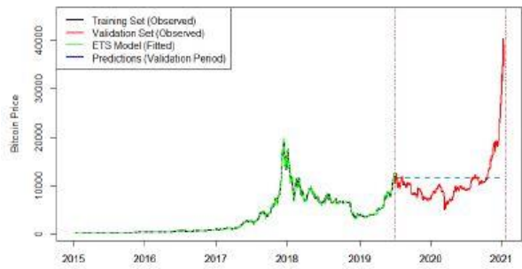
Figure 3c: Prediction in the validation period (ETS model)
