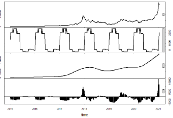
Figure 2b: STL decomposition of Bitcoin price (weekly)
