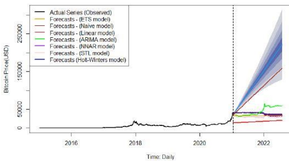
Figure 6g: Daily Bitcoin future forecasts (Holt-Winter model)
