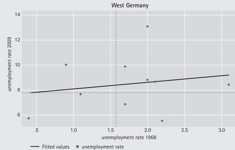
Figure 3.6: Persistence of West German regional unemployment rates, 1968–2009
