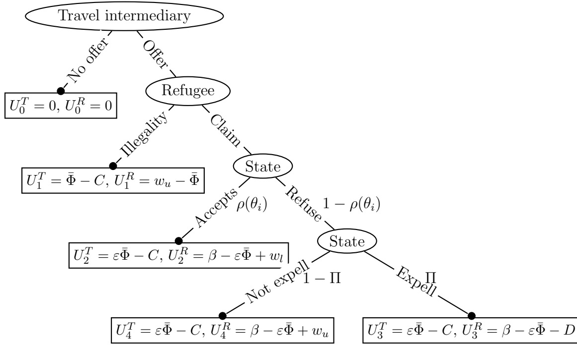
Figure 2: Game tree
