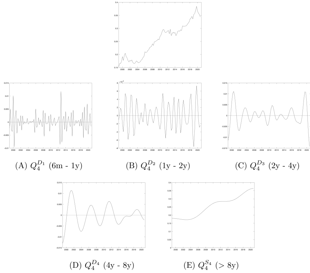
Figure C5: Time series of Q_4 and its decomposed components in Finland 1999Q1-2020Q4
