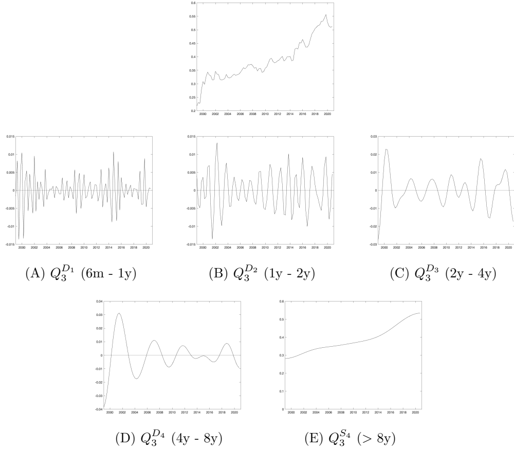
Figure C4: Time series of Q_3 and its decomposed components in Finland 1999Q1-2020Q4
