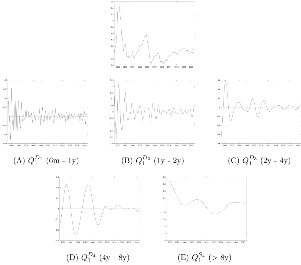
Figure C2: Time series of Q_1 and its decomposed components in Finland 1999Q1-2020Q4
