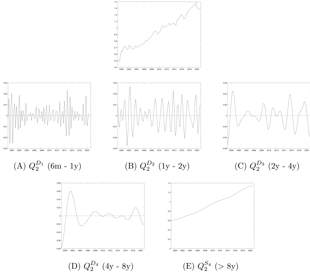
Figure C3: Time series Q_2 and its decomposed components in Finland 1999Q1-2020Q4
