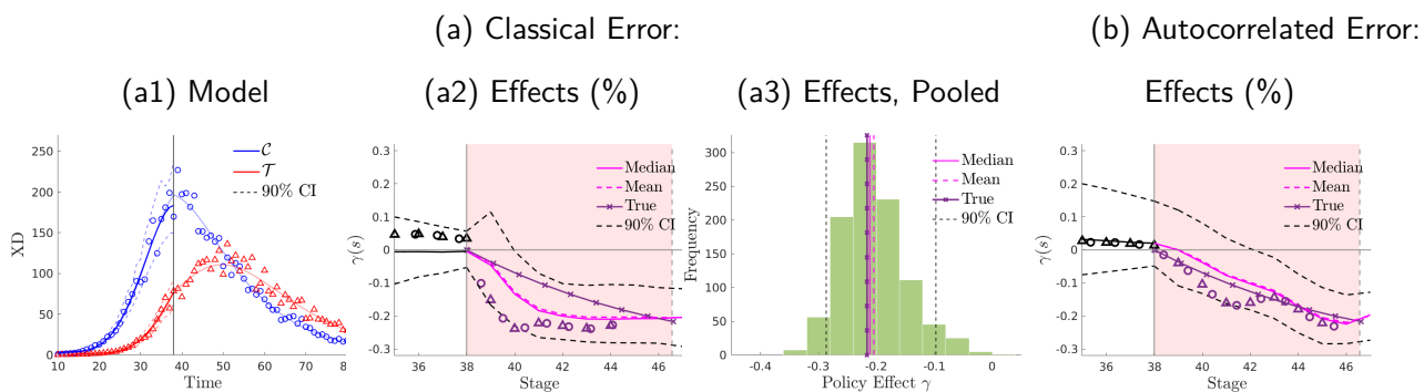
Figure 11: Stage-Based Identification of Model-Generated Policy Effects: Inference
