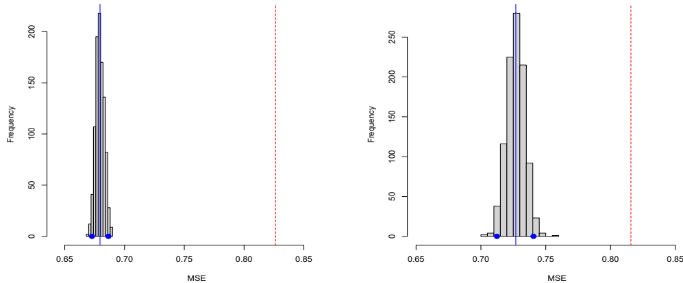
Figure A7: MSE posterior distribution for the BART(200) fitted on the sub-sample (grey bars), the average MSE (blue line), 95% HPD region (blue dots) and the MSE for the LASSO model (red dashed line). Left panel: in-sample. Right panel: out-of-sample.
