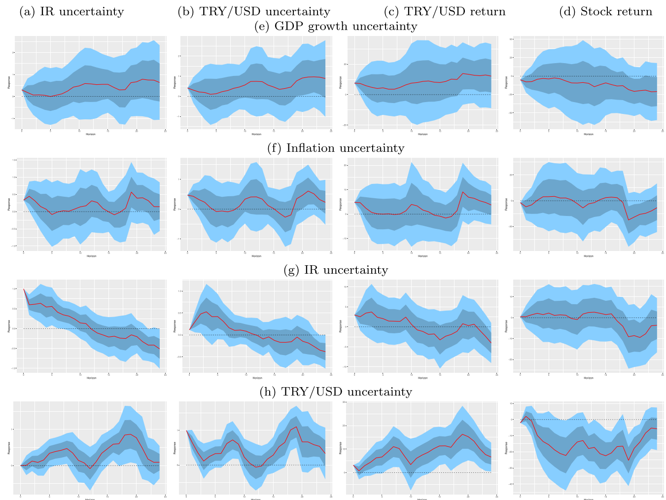
FIGURE 4 Orthogonalized impulse responses for the uncertainty model. The graphs show different orthogonalized impulse responses based on local projections for the uncertainty model. Uncertainty is proxied by the sum of ex post mean forecast error volatility and ex ante forecast disagreement for 12-month-ahead forecasts for each variable, and the model includes nine variables: Turkish GDP growth uncertainty, Turkish inflation uncertainty, US GDP growth uncertainty, US inflation uncertainty, Turkish short-term interest rate uncertainty, US short-term interest rate uncertainty, TRY/USD exchange rate uncertainty, realized percentage change of the TRY/USD exchange rate, and realized MSCI stock market returns for Turkey. Realized exchange rate changes and stock market returns are computed for a horizon of 12 months. The reaction is represented by the solid red line and the corresponding 95% (68%) confidence bands by blue (dark blue) shadings. The dashed black line displays the zero line. The impulses are one standard deviation shocks of the variables given in rows (e), (f), (g), and (h), and the response variables are given in columns (a), (b), (c), and (d). IR stands for 3-month interest rate.
