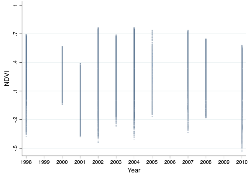
Figure 25: NDVI by cell and year (1998-2010)
