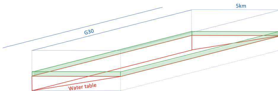
Figure 26: Depletion of the water table relative to G30
