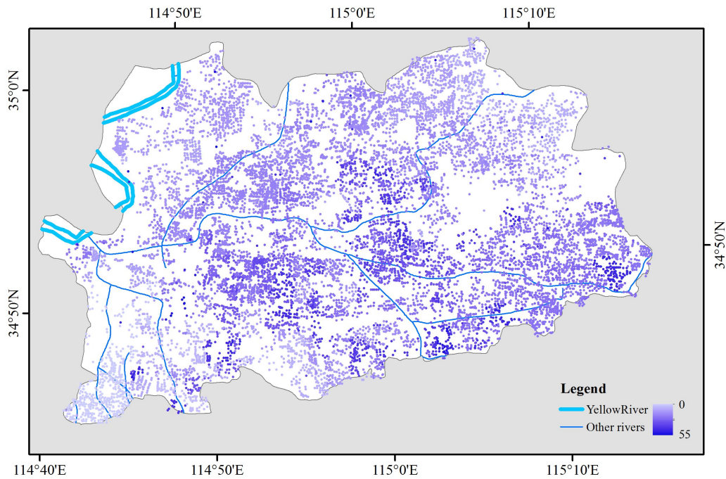
Figure 8: Depth of water table in tubewells in 2011
