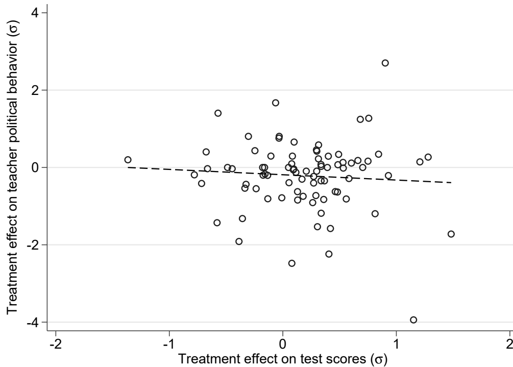
Scatter plot of treatment effects on student test scores and an index of teacher political behavior, measured at the level of school pairs. N = 83 pairs for which treatment effects for both variables are measurable. Correlation = -0.074
