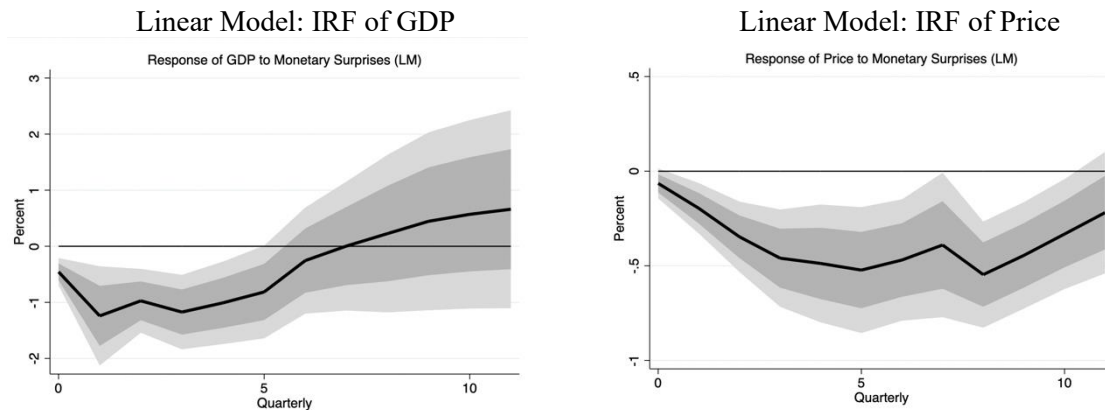
Figure 2: Linear Models
