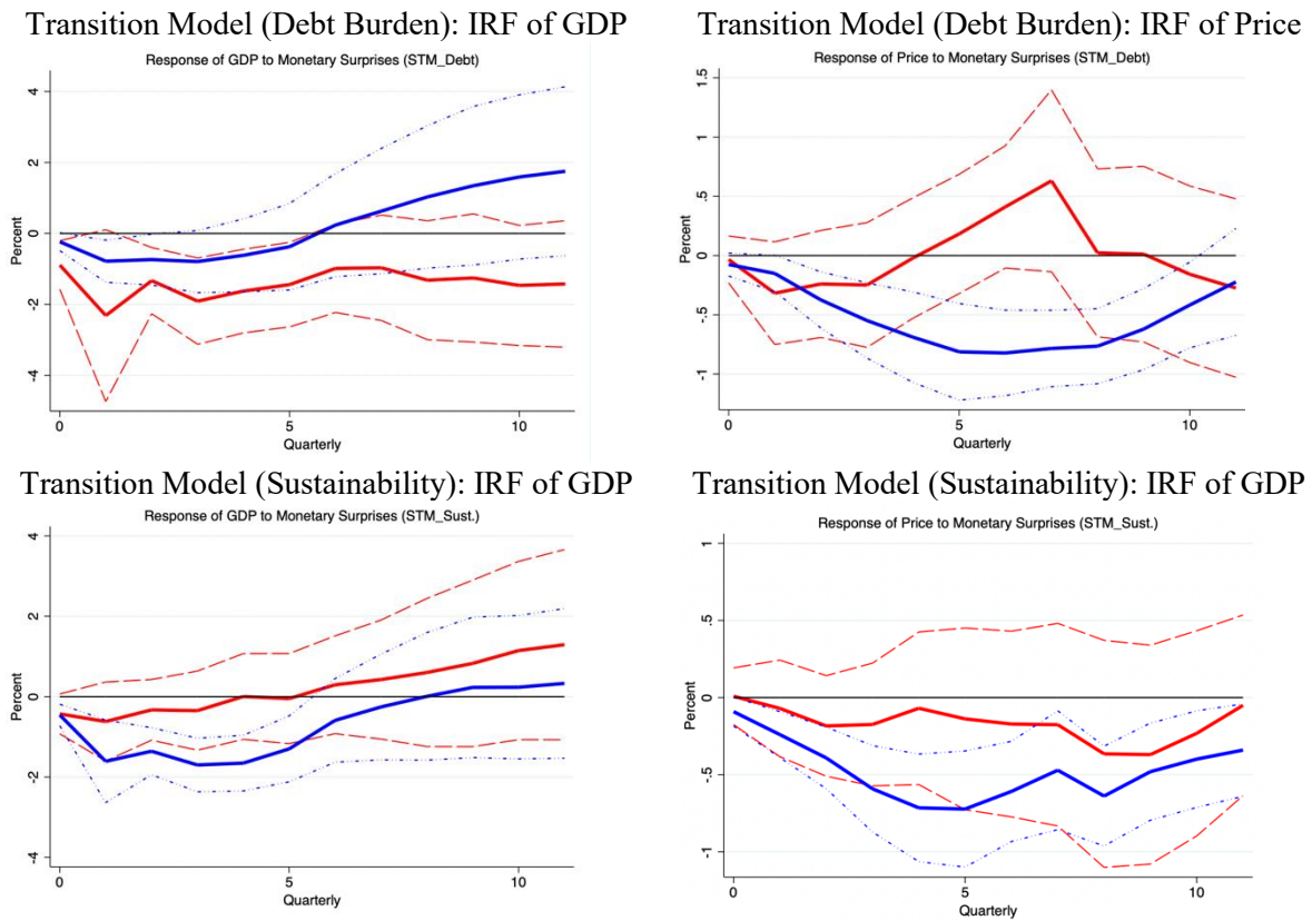
Figure 4: Transition Model
