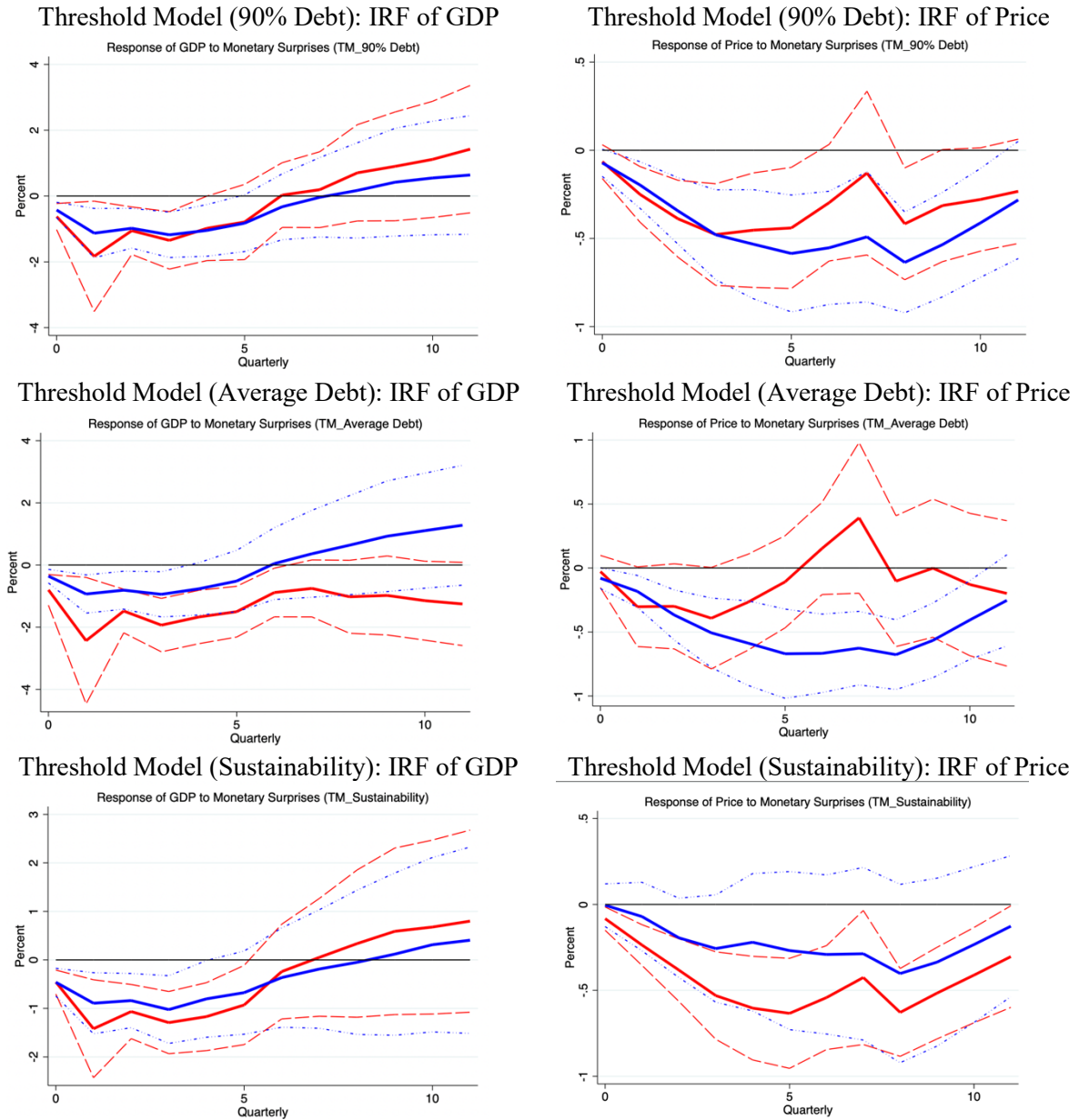
Figure 3: Threshold Model
