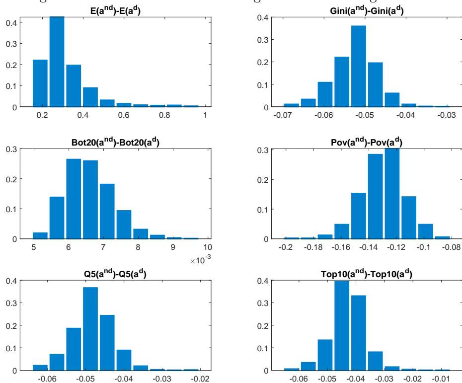
Figure D1: Monte Carlo exercise
