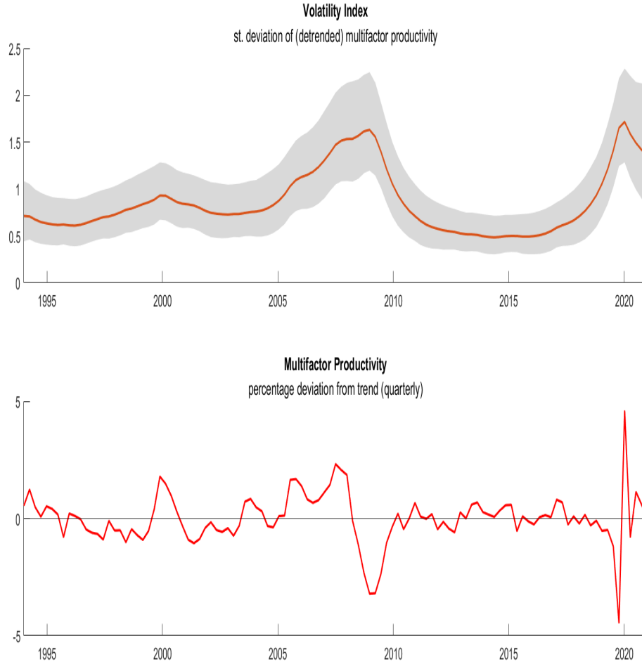
Figure 5: Volatility Index
