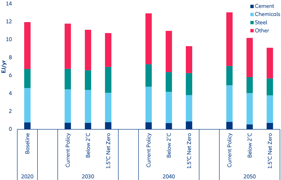
Figure 4: Final energy use by sector and scenario
