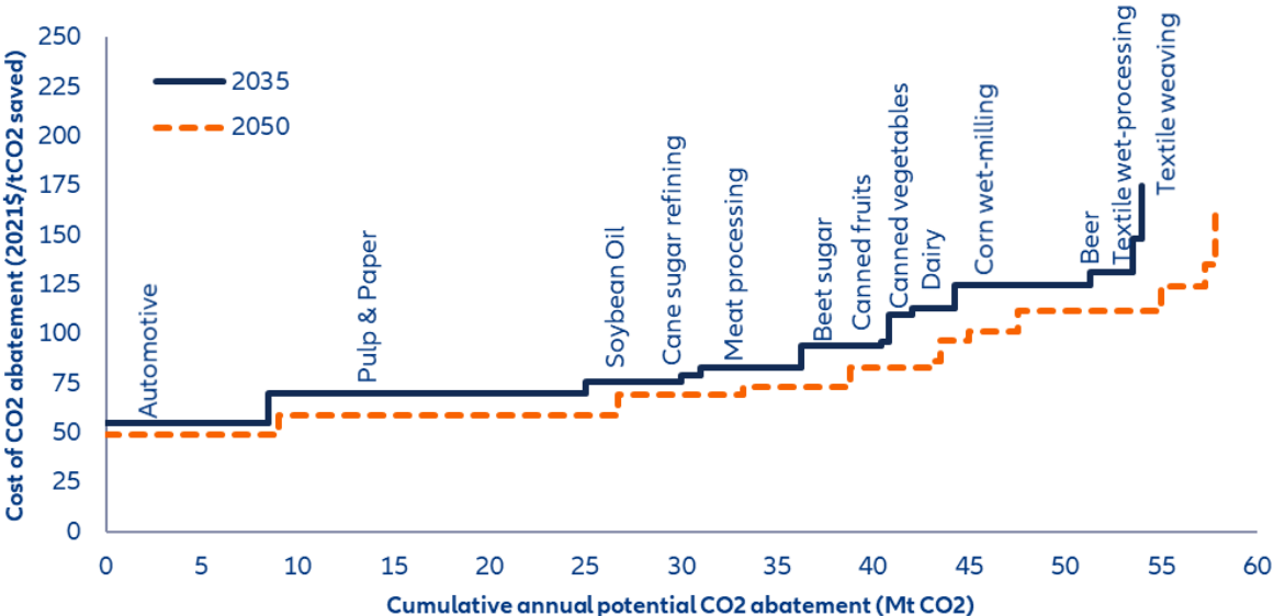
Figure 5: CO 2 abatement potentials through heat pumps in US manufacturing
