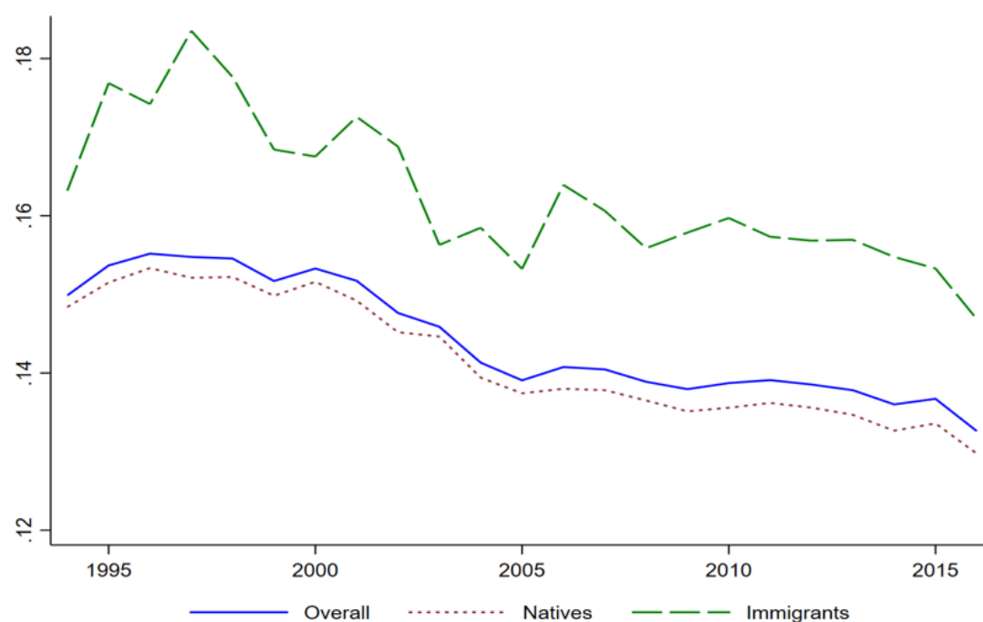
FIGURE 16. Theil index
