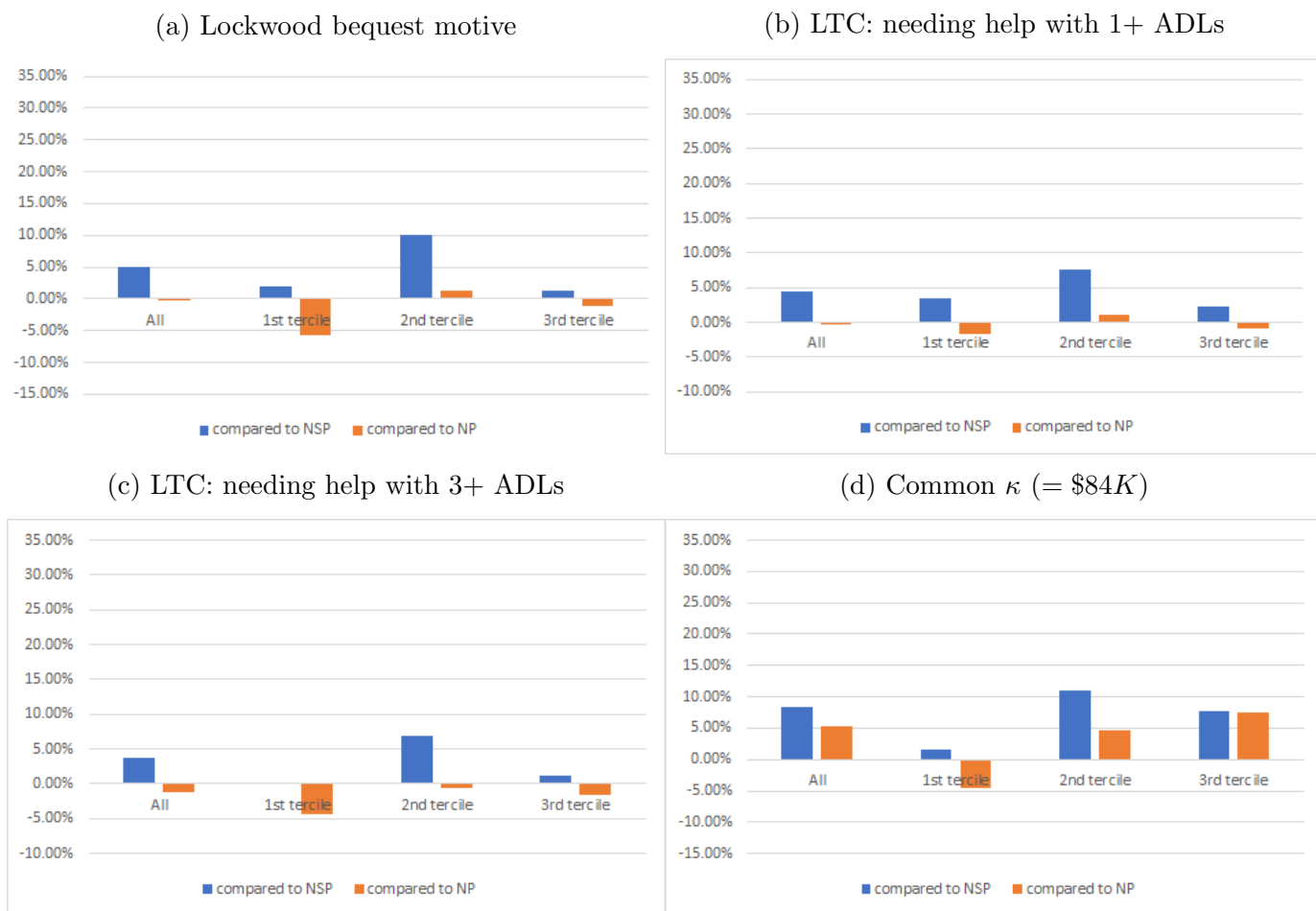
Figure E2: Additional savings by HC under means-tested only (%): age 66, alternative specifications
