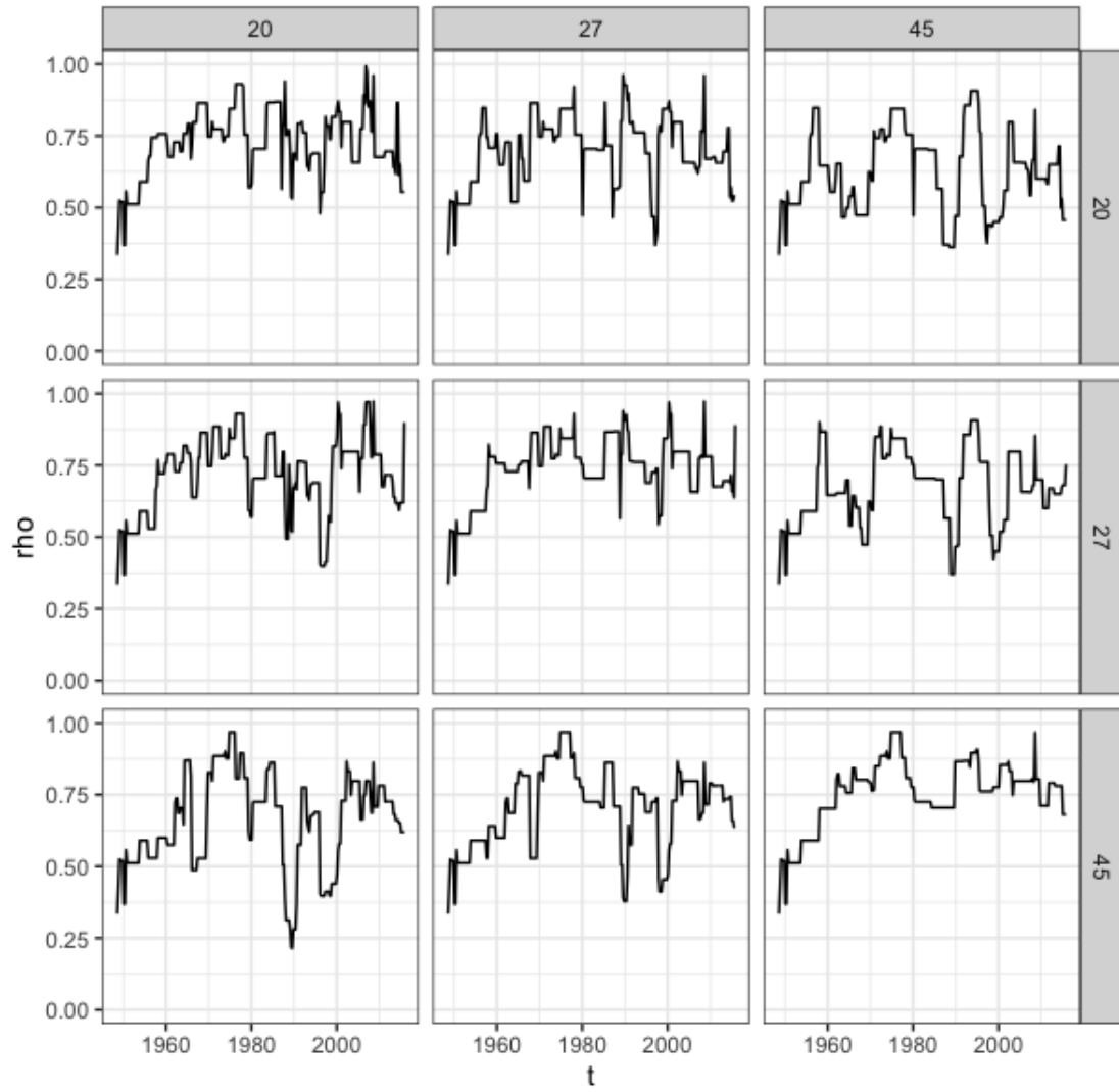
Figure 5: TPMA (main diagonal) and MTPMA (off-diagonal) for growth rates of per capita GDP and consumption.
