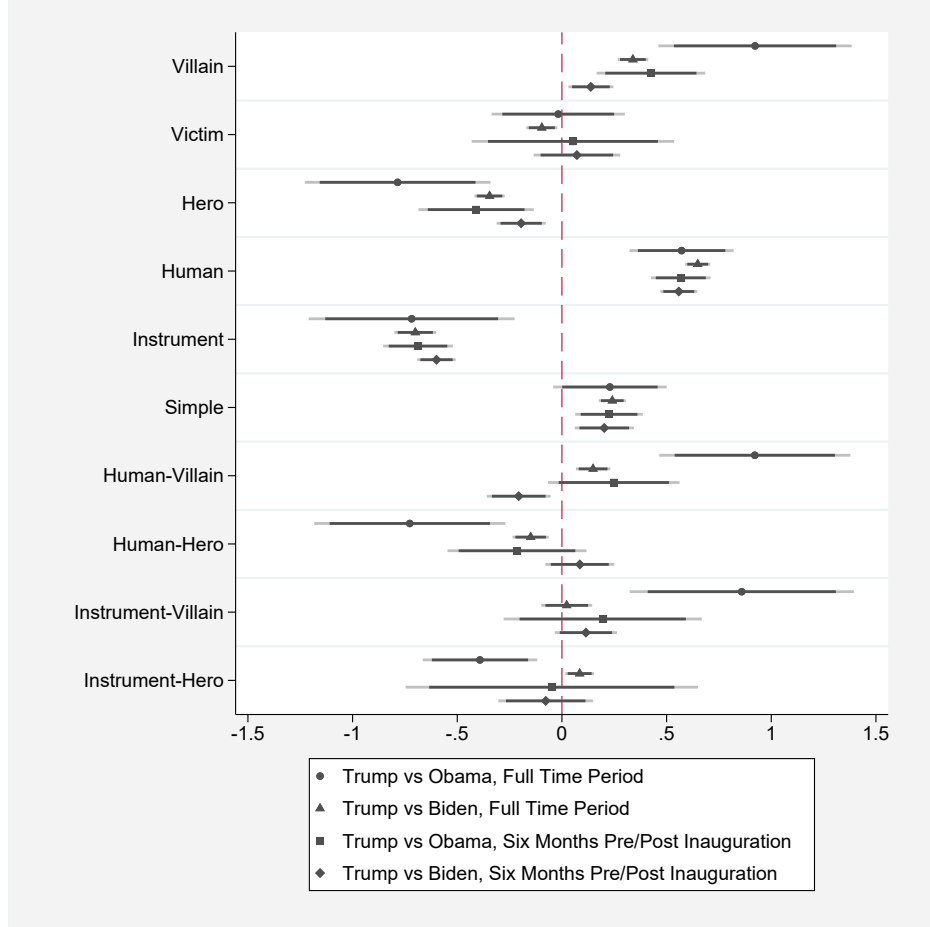
Figure E.7: The Trump Effect - Logistic Regression
