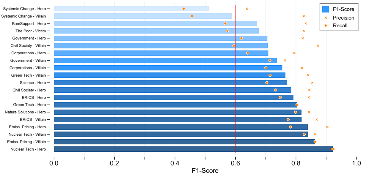
Figure 3: Model Performance by Character-Role
