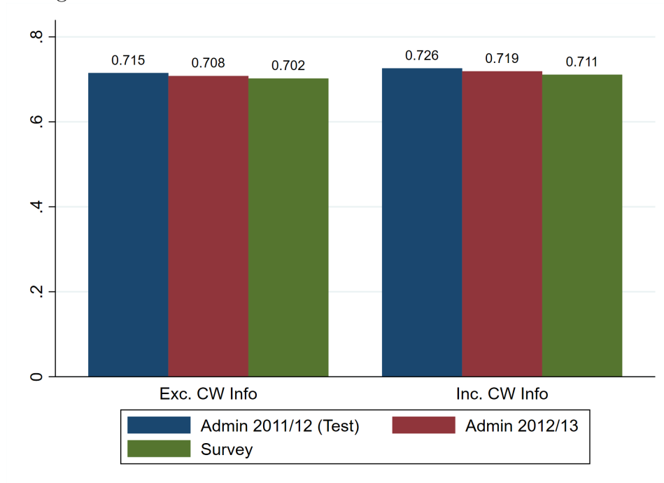
Figure A 2: ROC-AUC Scores with and without caseworker info
