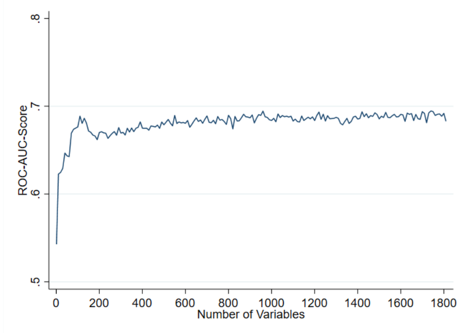
Figure B 1: ROC-AUC for an increasing number of variables - admin, no CW info
