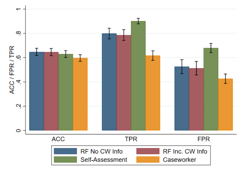
Figure 2: Accuracy, TPR, and FPR of the four predictors at a threshold of 0.5
