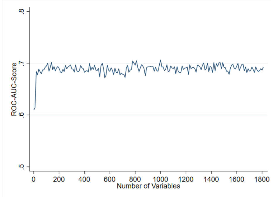
Figure A 7: ROC-AUC for an increasing number of variables - survey, inc. CW info
