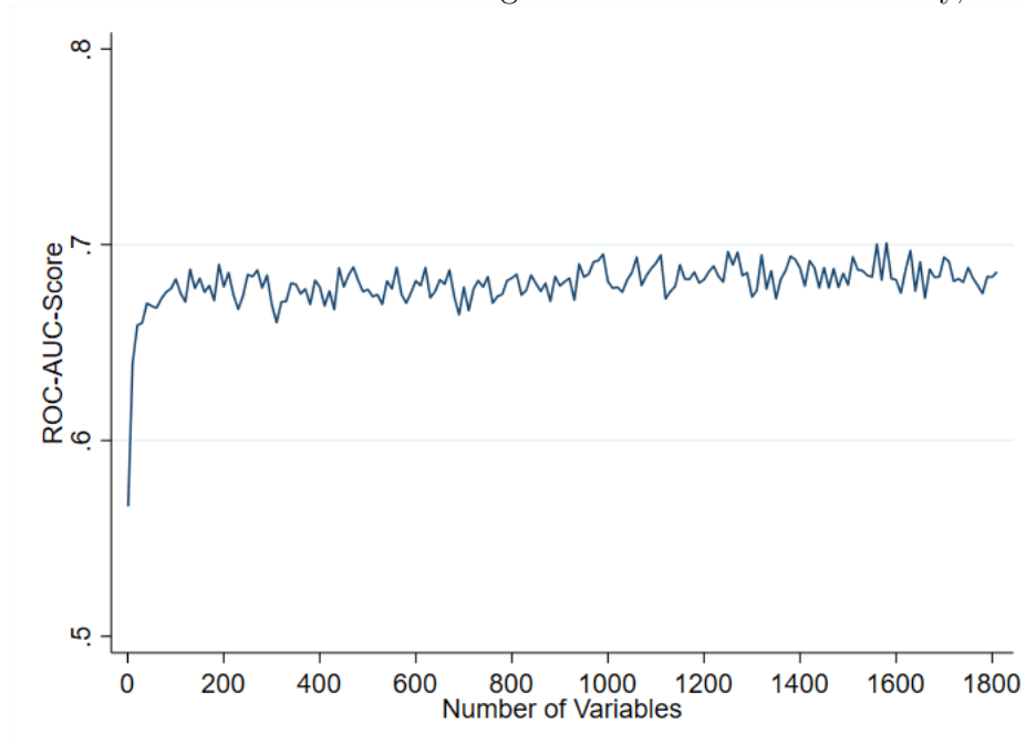
Figure A 6: ROC-AUC for an increasing number of variables - survey, no CW info
