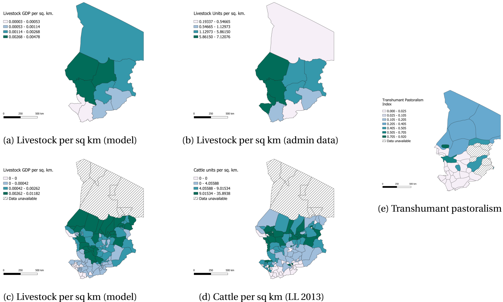
Figure E.9: Validation of the Model: Livestock Distribution in Chad c. 1963
