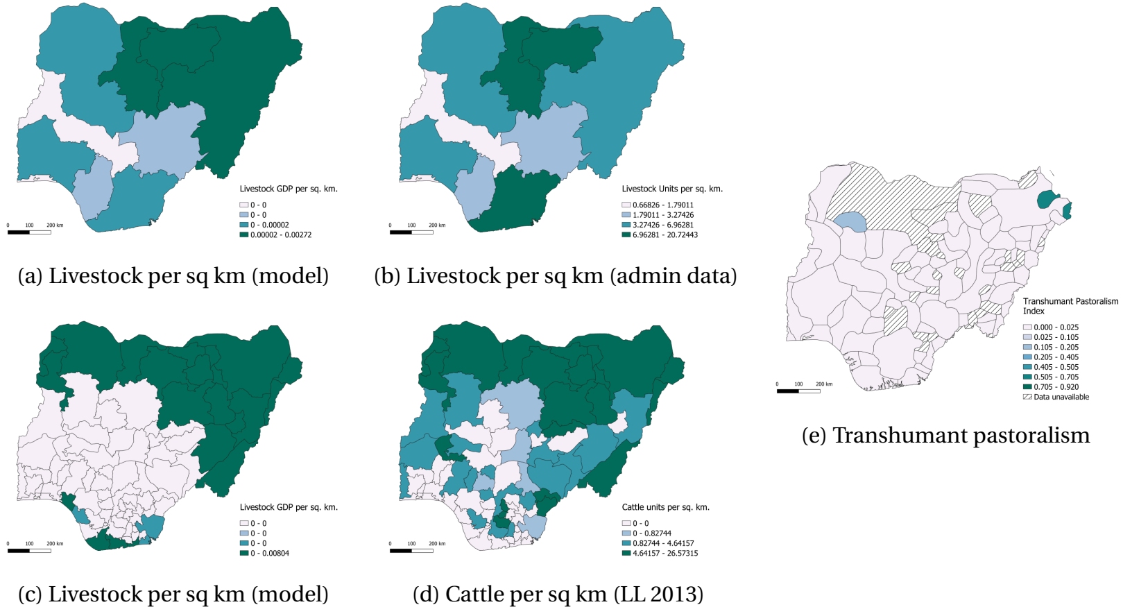
Figure E.11: Validation of the Model: Livestock Distribution in Nigeria c. 1963
