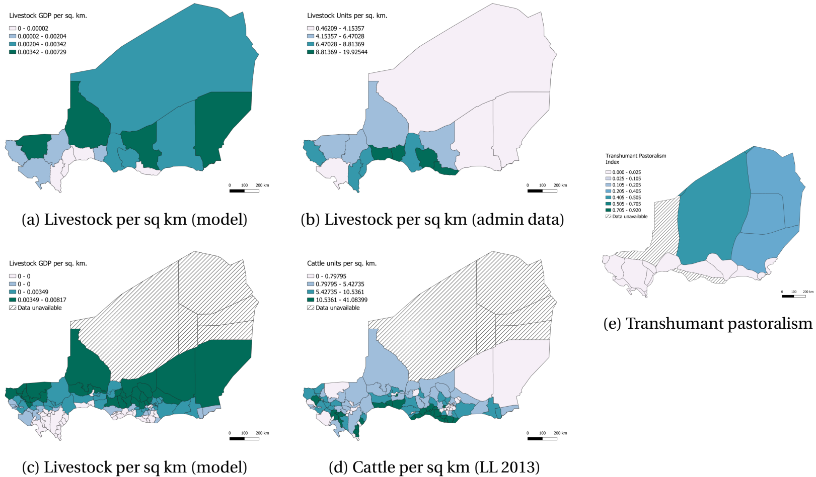
Figure E.10: Validation of the Model: Livestock Distribution in Niger c. 1963
