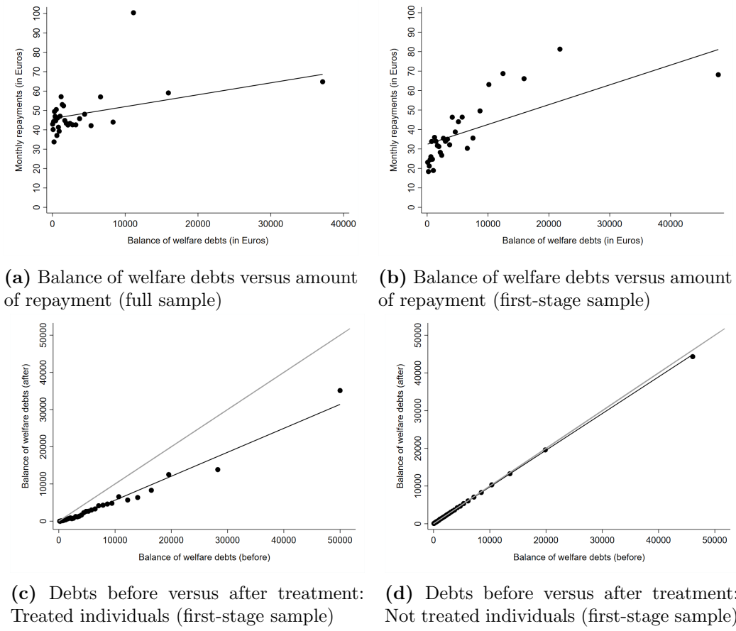
Figure 2: Binscatter plots
