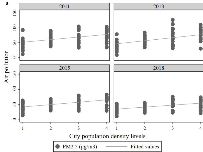
Fig. A1 Variations in Annual Mean Air Pollution and City Population Density Levels
