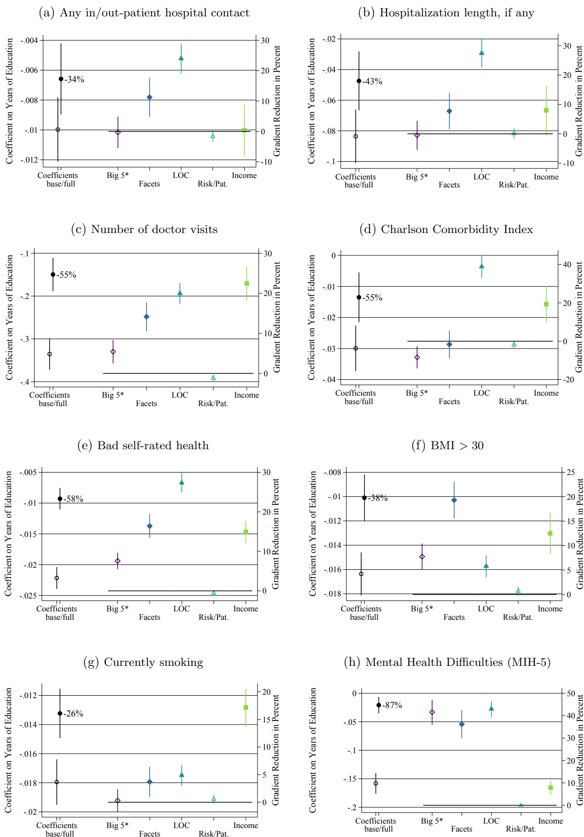
Figure 5: Gradient Reductions
