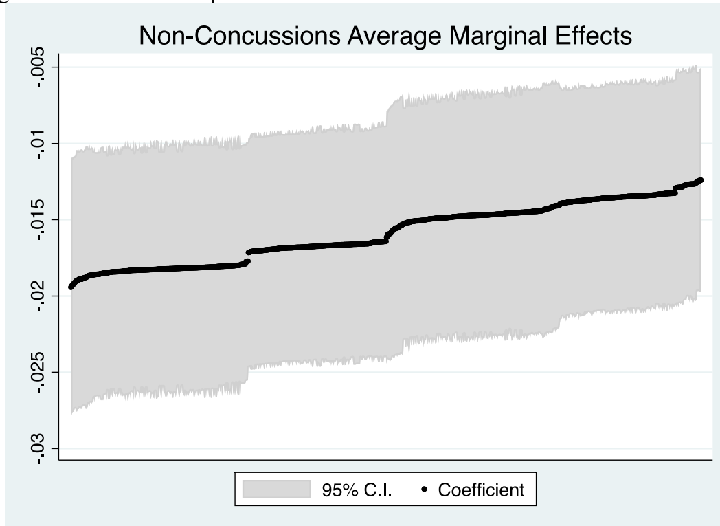
Figure A6. Performance Specifications- Concussions and Non-Concussions Estimations
