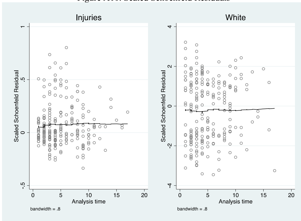
Figure A10. Scaled Schoenfeld Residuals
