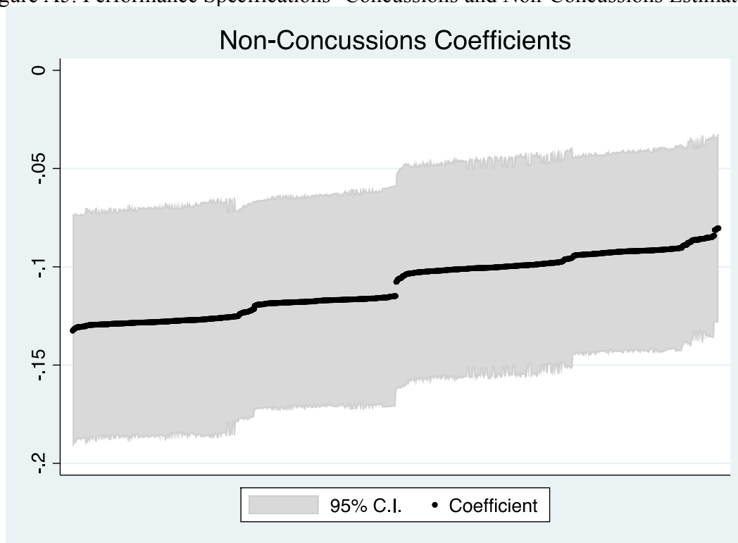
Figure A5. Performance Specifications- Concussions and Non-Concussions Estimations
