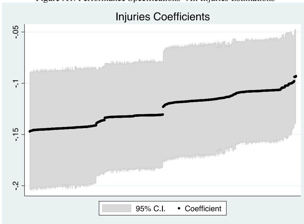
Figure A1. Performance Specifications- All Injuries Estimations
