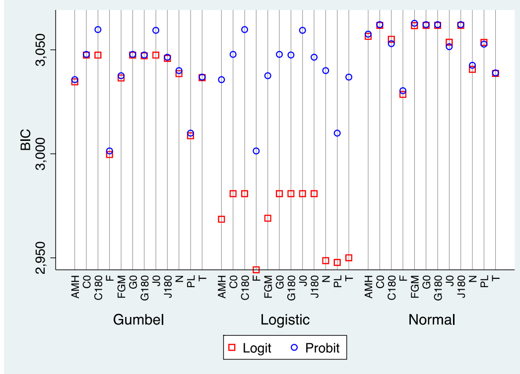
Figure A14. Copula Model Comparison- Concussions and Non-Concussion Injuries
