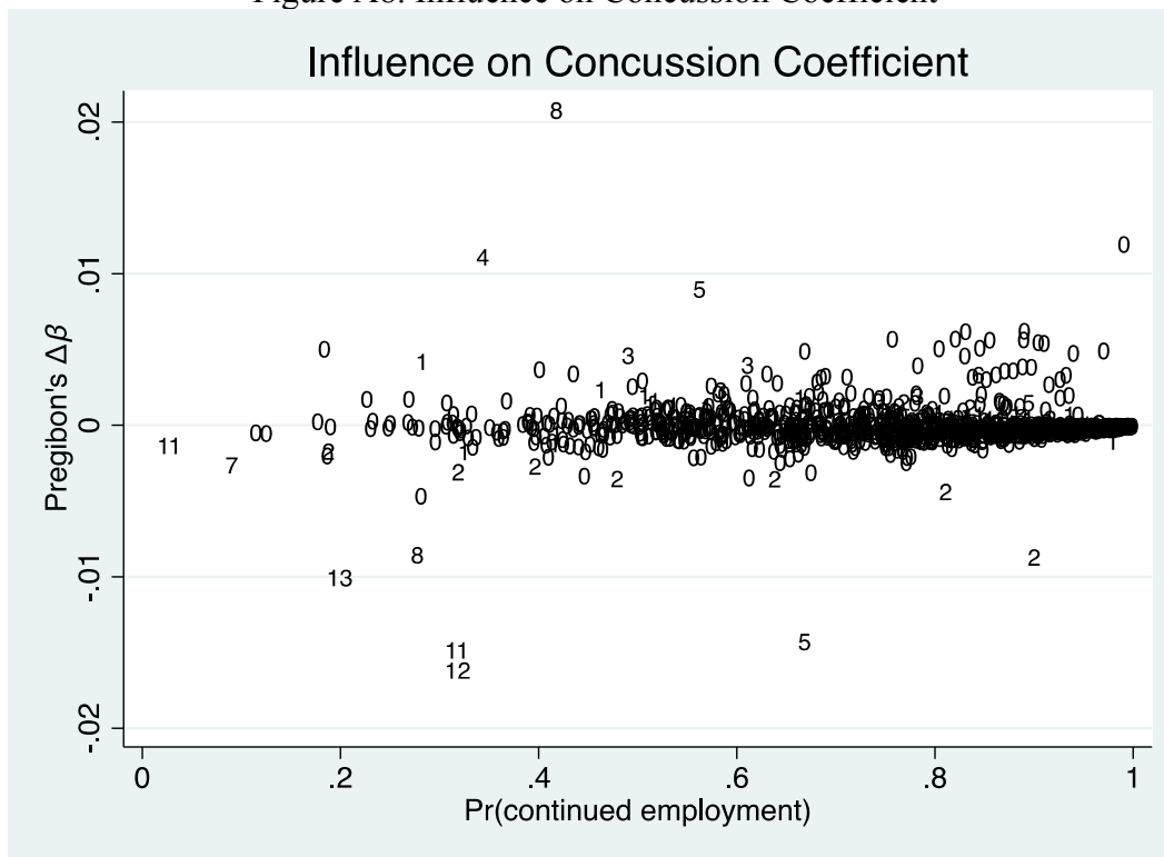
Figure A8. Influence on Concussion Coefficient
