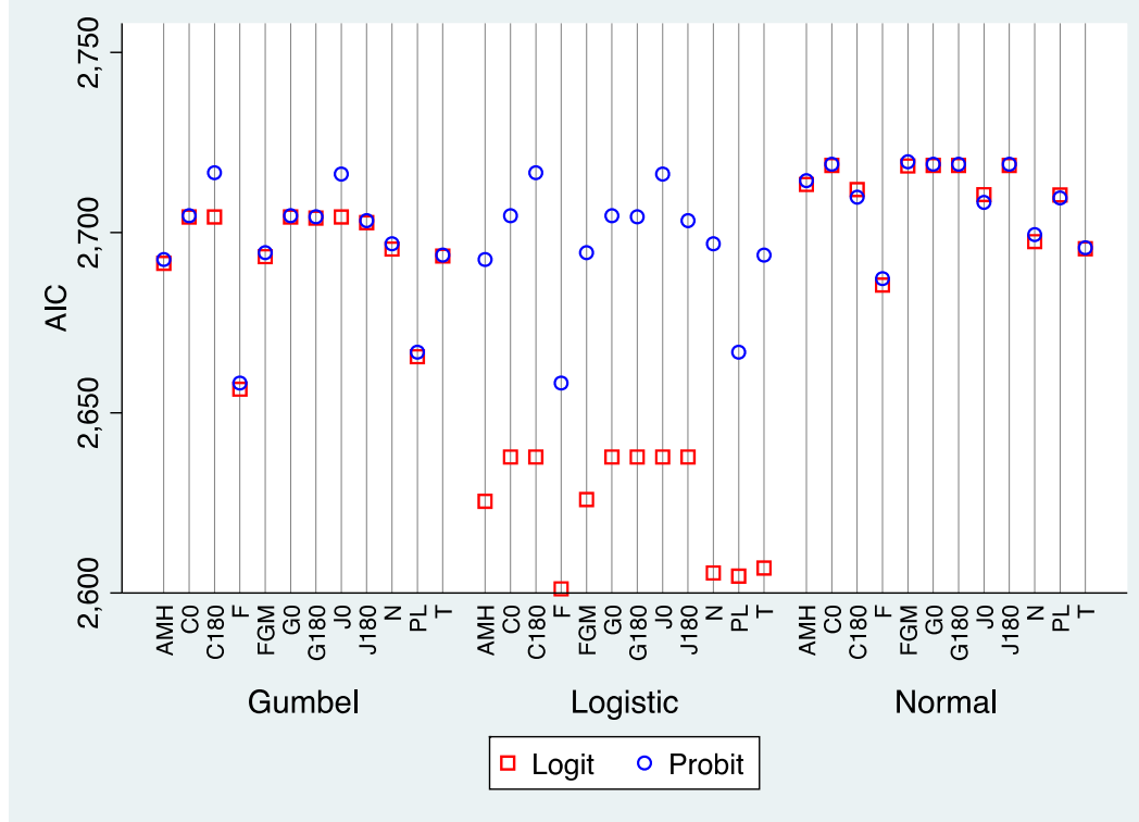
Figure A13. Copula Model Comparison- Concussions and Non-Concussion Injuries
