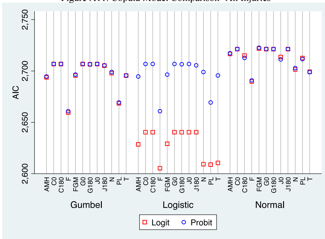
Figure A11. Copula Model Comparison- All Injuries
