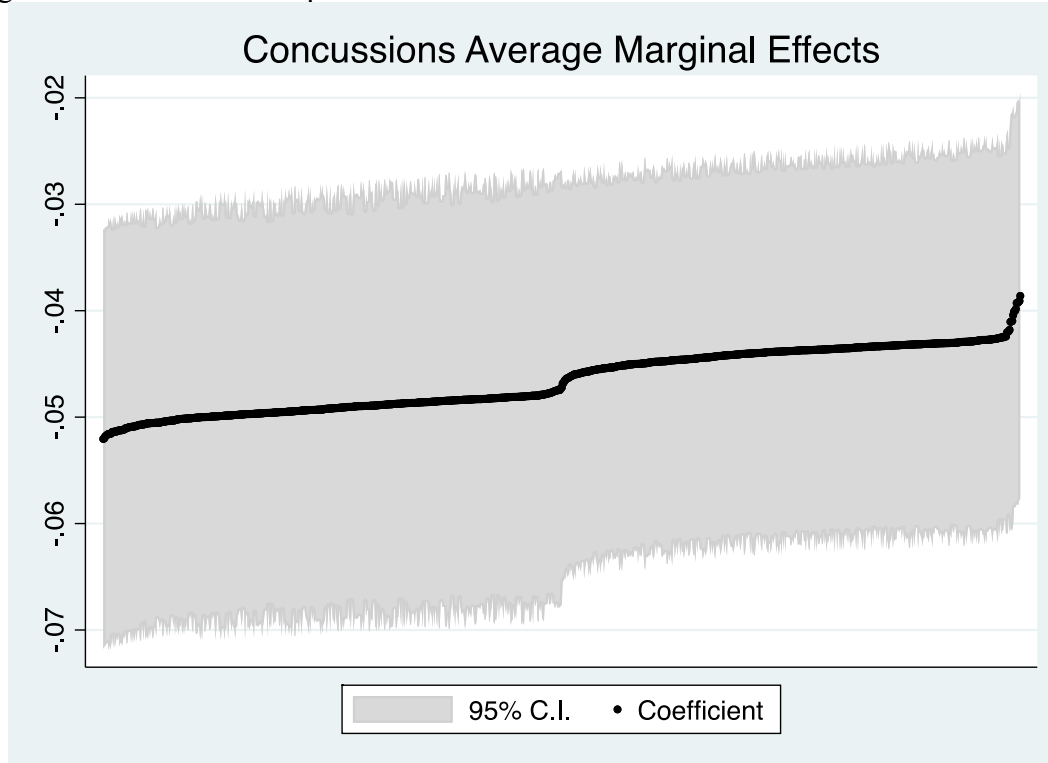
Figure A4. Performance Specifications- Concussions and Non-Concussions Estimations
