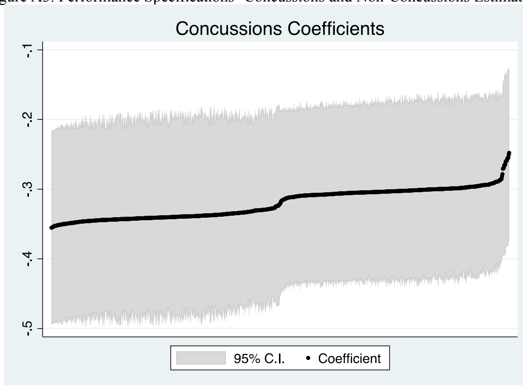
Figure A3. Performance Specifications- Concussions and Non-Concussions Estimations
