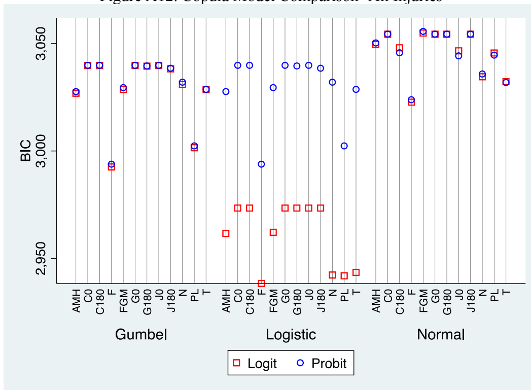
Figure A12. Copula Model Comparison- All Injuries
