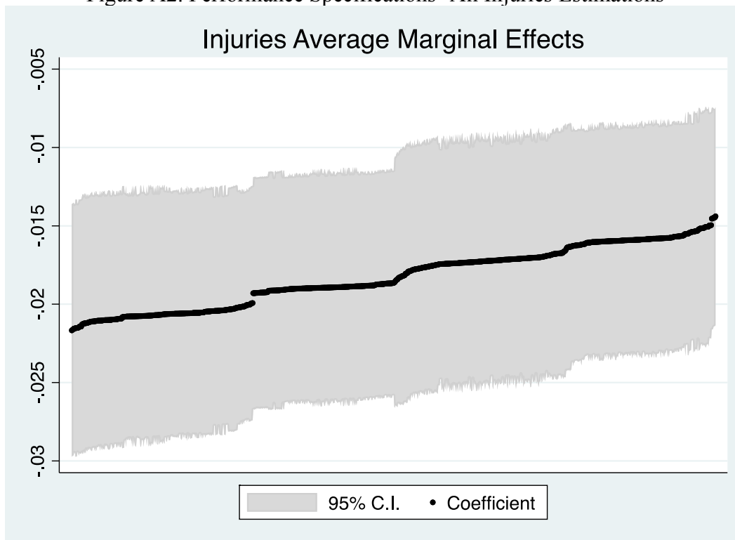
Figure A2. Performance Specifications- All Injuries Estimations
