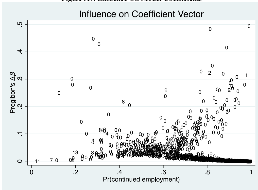
Figure A7. Influence On Model Coefficients
