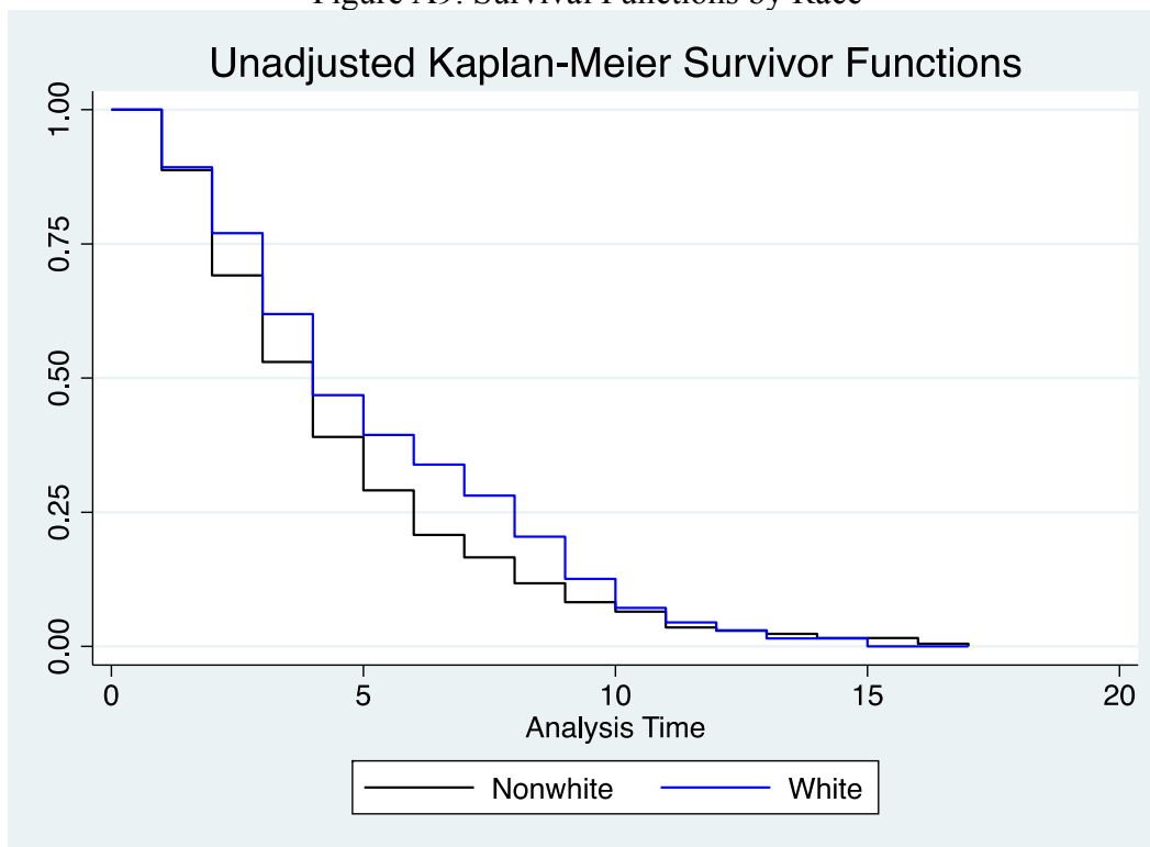
Figure A9. Survival Functions by Race
