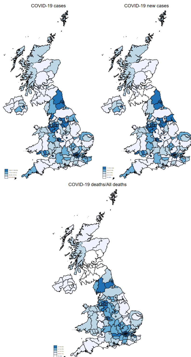
Figure 3: Geographical variability for the ratio between COVID-19 deaths and deaths for other causes.
