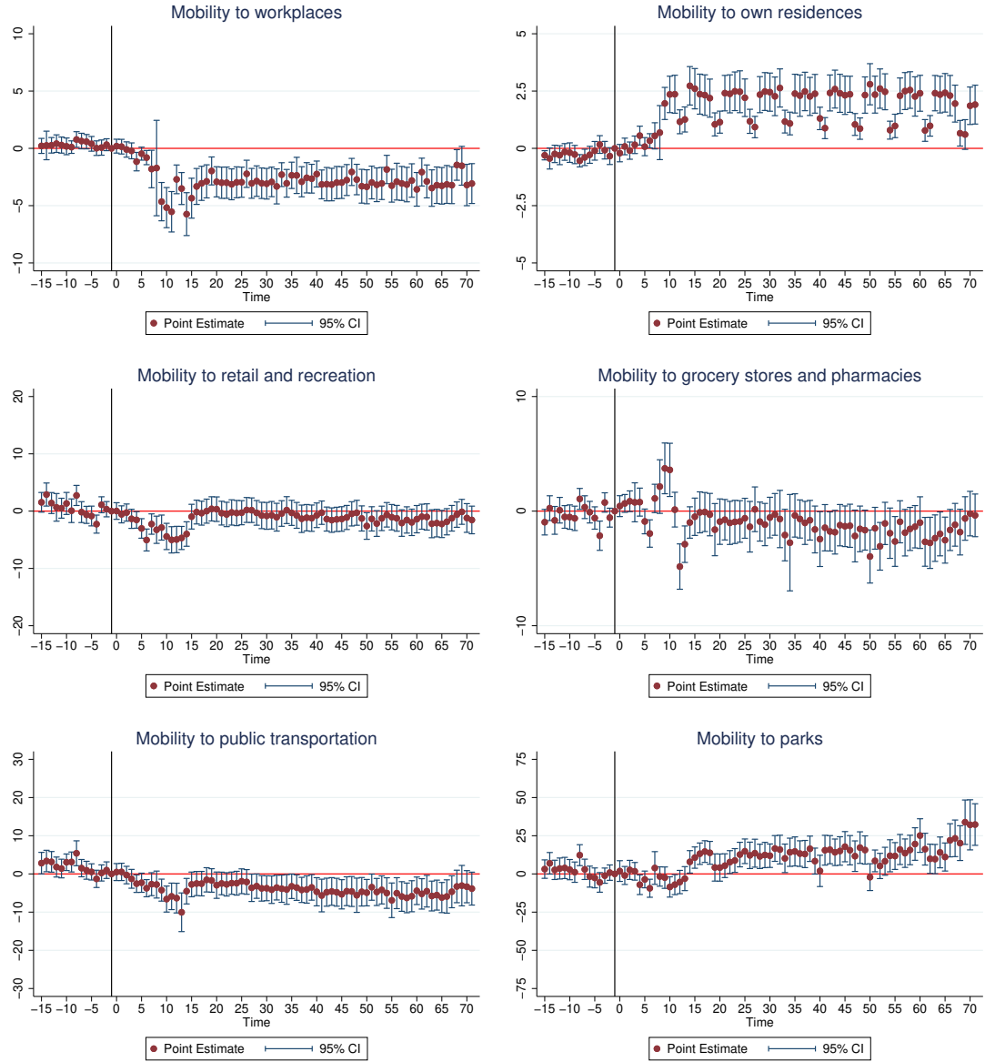
Figure 7: event estimates of the effect of living, during the UK COVID-19 restrictions, in regions with the ratio between COVID-19 deaths and deaths for other causes higher than the country average on mobility.
