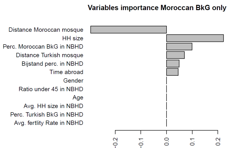
Figure A6: Penalized Logit model coefficients: Moroccan BkG
