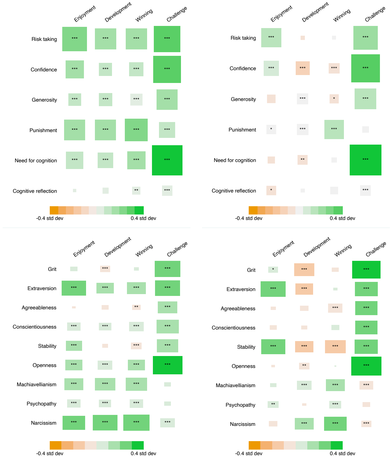
Figure 3: Conditional correlations between competitiveness and other psychological traits
