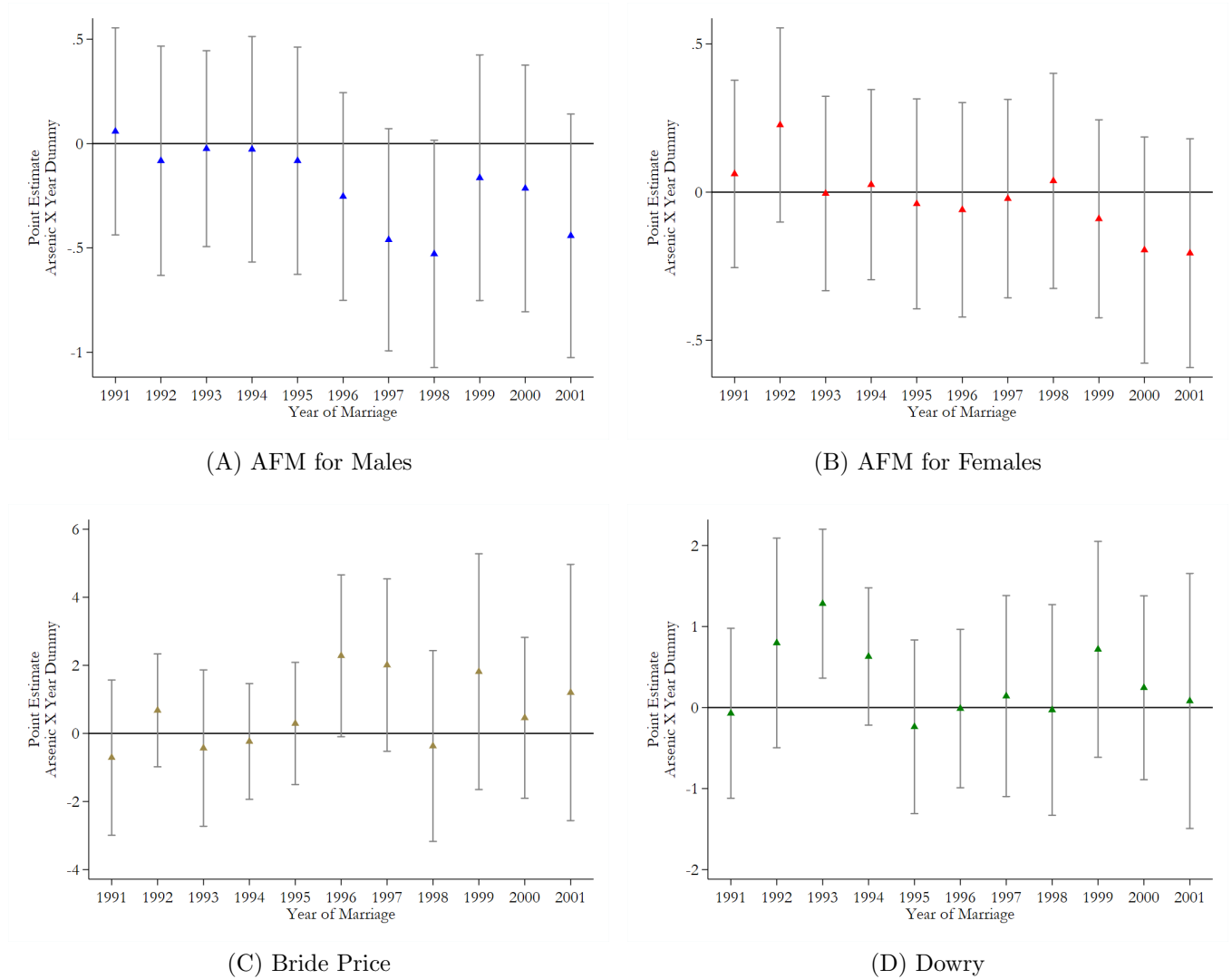
Figure A3: Testing for Parallel Trend Assumption.
