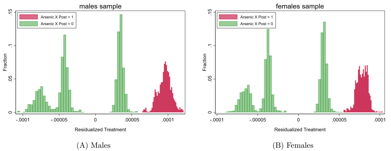
Figure A4: Weights in Two-way Fixed Effects Regressions
