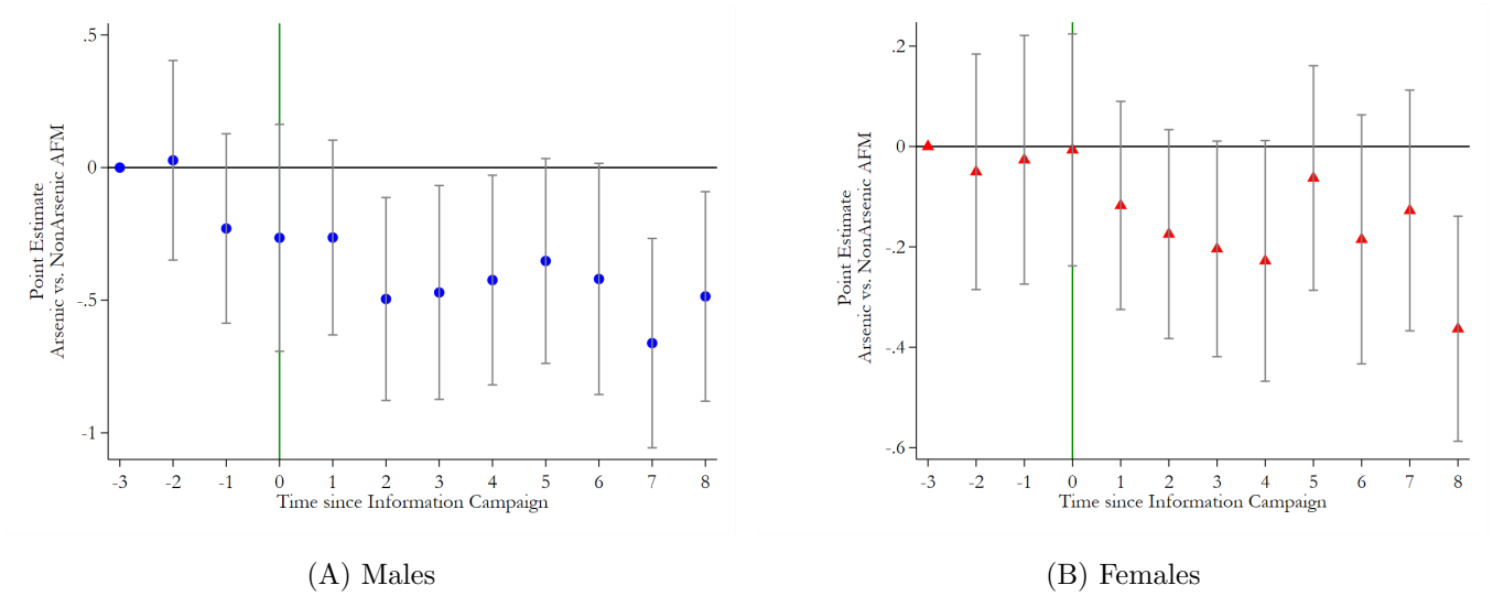
Figure 4: Event Study Analyses
