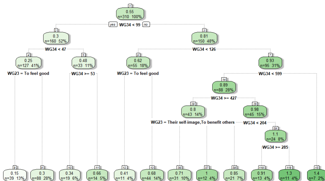
Figure 2: Large regression tree for predicting WG9
