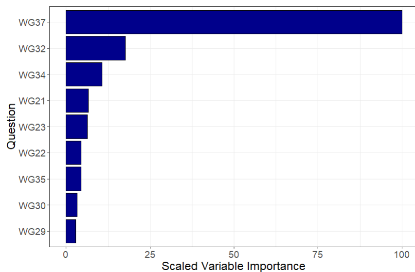
Figure 4: Variable Importance Plot for the random forest modeling Donation Amount in WG9
