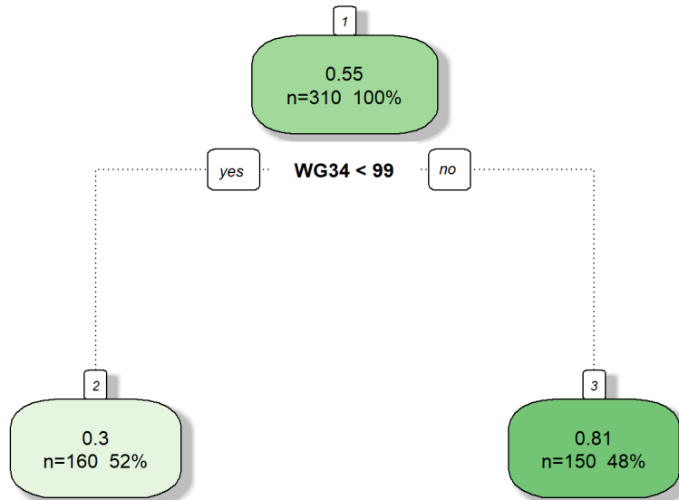
Figure 1: A one-step regression tree for survey data
