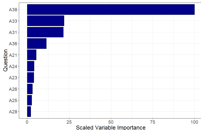
Figure 3: Variable Importance Plot for the random forest modeling Donation Amount in A14
