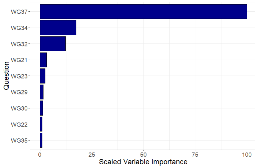
Figure 8: Variable Importance Plot for the random forest modeling WG9_Donated
