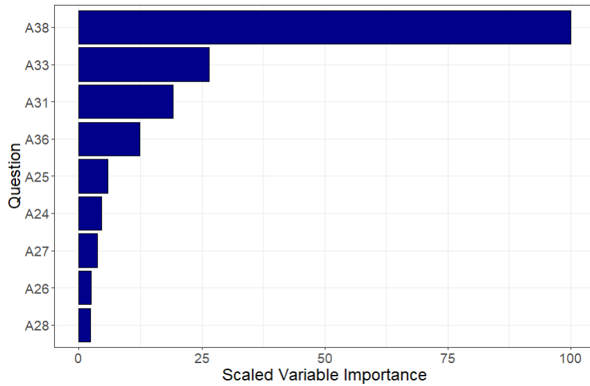
Figure 7: Variable Importance Plot for the random forest modeling A14_Donated
