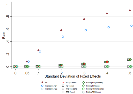
FIGURE A.7: Simulation Results: Bias
