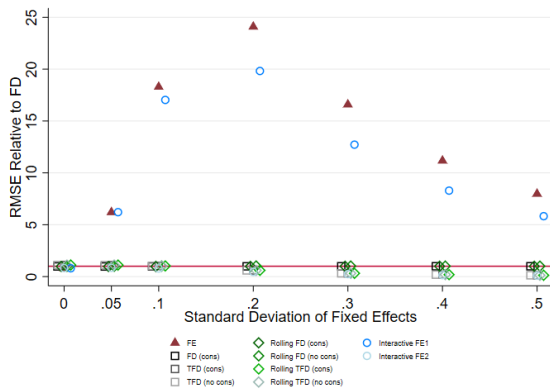
FIGURE A.6: Simulation Results: Root Mean Squared Error
