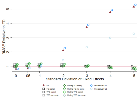
FIGURE A.2: Simulation Results: Root Mean Squared Error
