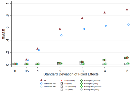
FIGURE A.8: Simulation Results: Root Mean Squared Error
