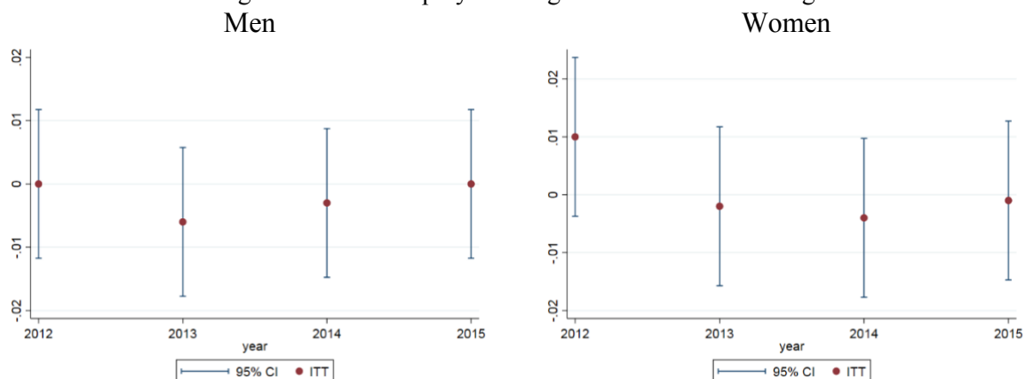
Figure 6. Pre-treatment trend: Regression discontinuity estimates at the 30-years of age threshold and their confidence intervals for outcomes 36 months after registration in the years 2012-2015, by gender.
