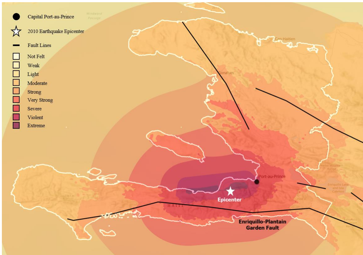
Figure A1. USGS ShakeMap of the 2010 Haiti Earthquake
