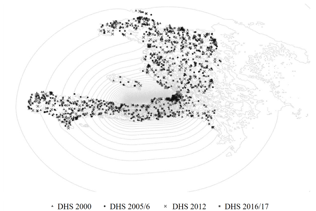
Figure 3. USGS ShakeMap Haiti together with DHS clusters
