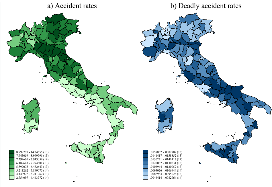
Figure A.1: Work related daily accident rates per 100,000 workers averaged over 2008–2021
