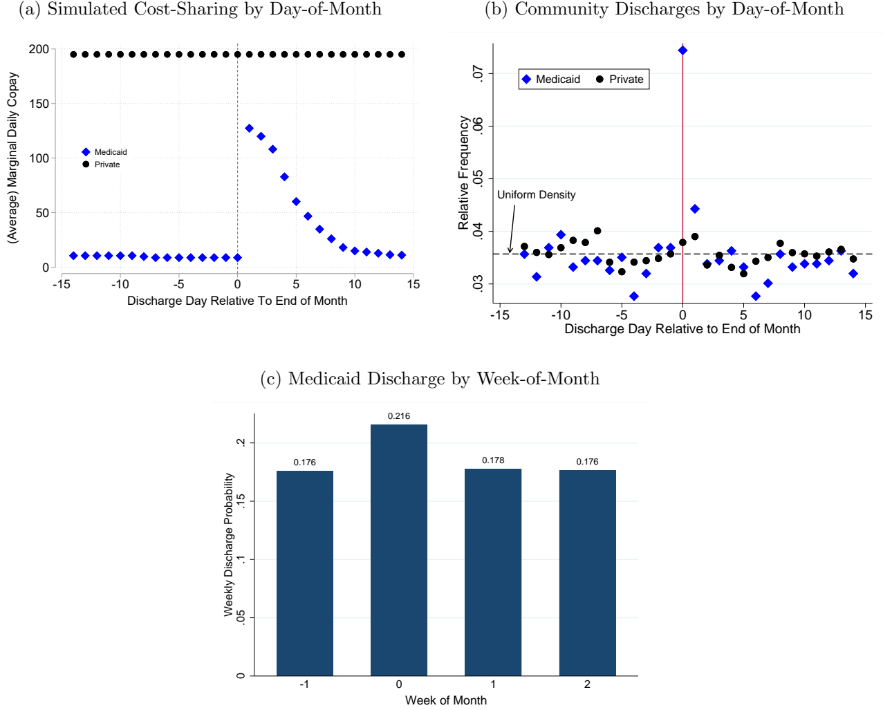
Figure E.10: Daily Cost-Sharing and Community Discharges—Bunching Analysis
