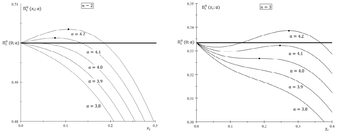
Figure 1. Expected payoff against inactive opponents.
