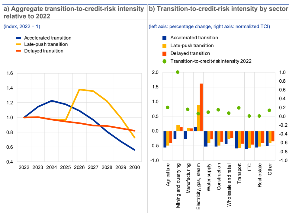
Chart 30 Transition-to-credit-risk intensity across time and sectors
