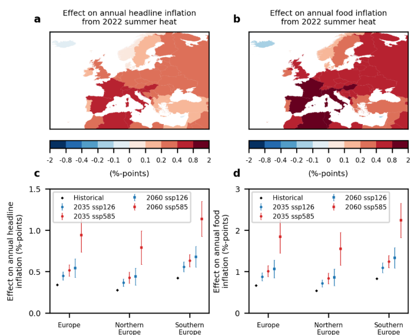
Figure 4. Estimated impacts of 2022 summer extreme heat in Europe on inflation, and the amplification of impacts from such extremes under projected future warming. (a) The cumulative impacts on headline (a) and food (b) inflation from the observed temperatures of June, July and August of 2022 across Europe. Regionally aggregated (using a population weighting) impacts on headline (a) and food (b) inflation from the historical 2022 summer temperatures, as well as those impacts which would result from such a summer when amplified by future warming (see section 2.7). Future warming by 2035 and 2060 are estimated as the difference between 30-year averages centred on the respective future time-points and 2022, using climate models of the CMIP-6 ensemble under both low (SSP126) and high (SSP585) emission scenarios. Point estimates and error bars show the mean and standard deviation of impacts across climate models.
