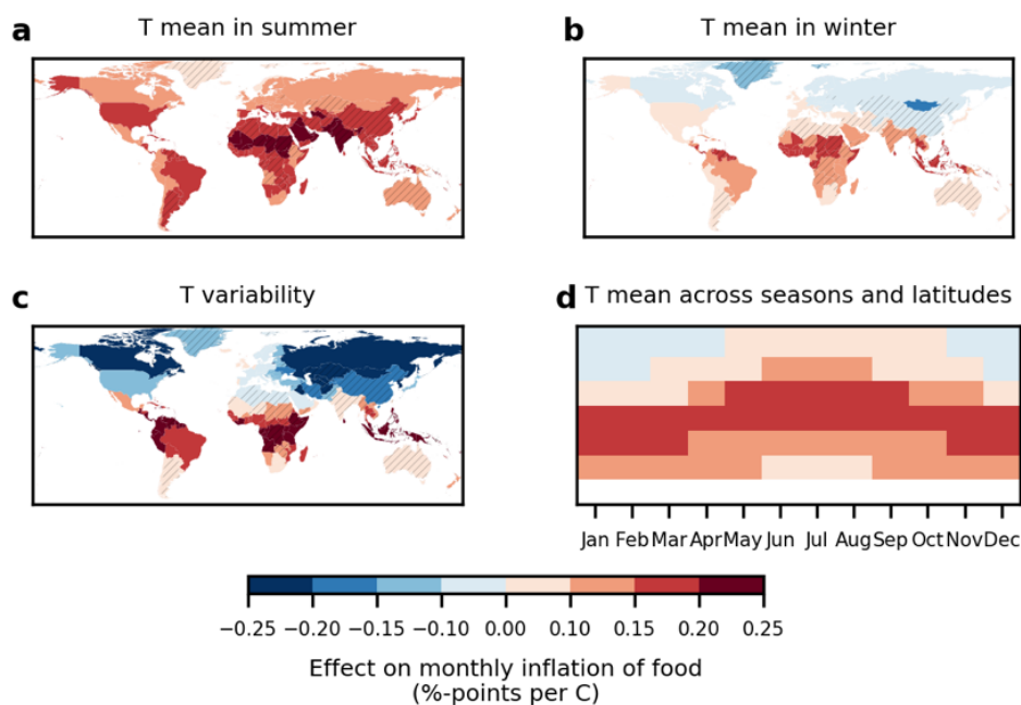
Figure S1. The historically observed non-linear response of inflation to temperature across regions and seasons. The cumulative response over 12 months of food inflation to a 1C increase in monthly mean temperature when occurring in either the hottest month of that countries year (a) or the coldest month of that countries year (b). The response to mean temperature increases in each separate month of the year, aggregated across latitudinal zones is shown in (d). The equivalent response of inflation to a 1C increase in daily temperature variability in any month of a given country (c). Estimates are extrapolated to regions without data on consumer price indices by evaluating the marginal effects estimated in Fig. 1 at the values of the moderating variable (either mean temperature or the magnitude of the seasonal temperature cycle) for each country.
