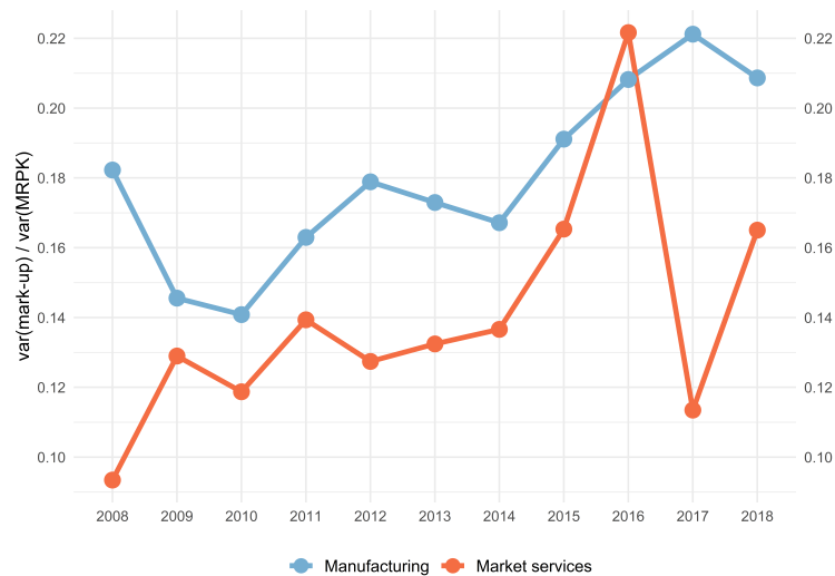
Figure 5: Development of the share of variation in MRPK explained by variation in mark-ups, industry aggregates
