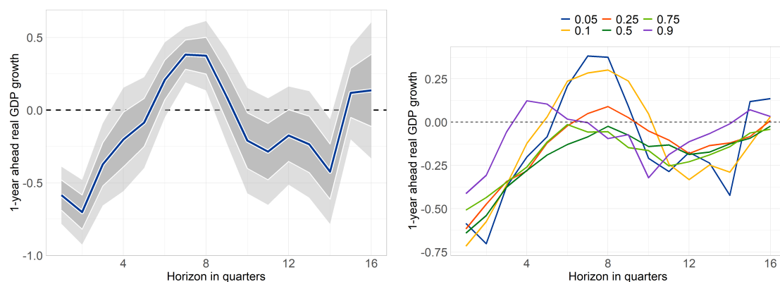
Figure A2: QIRFs for Debt Service Ratio (full model, no fixed effects)
