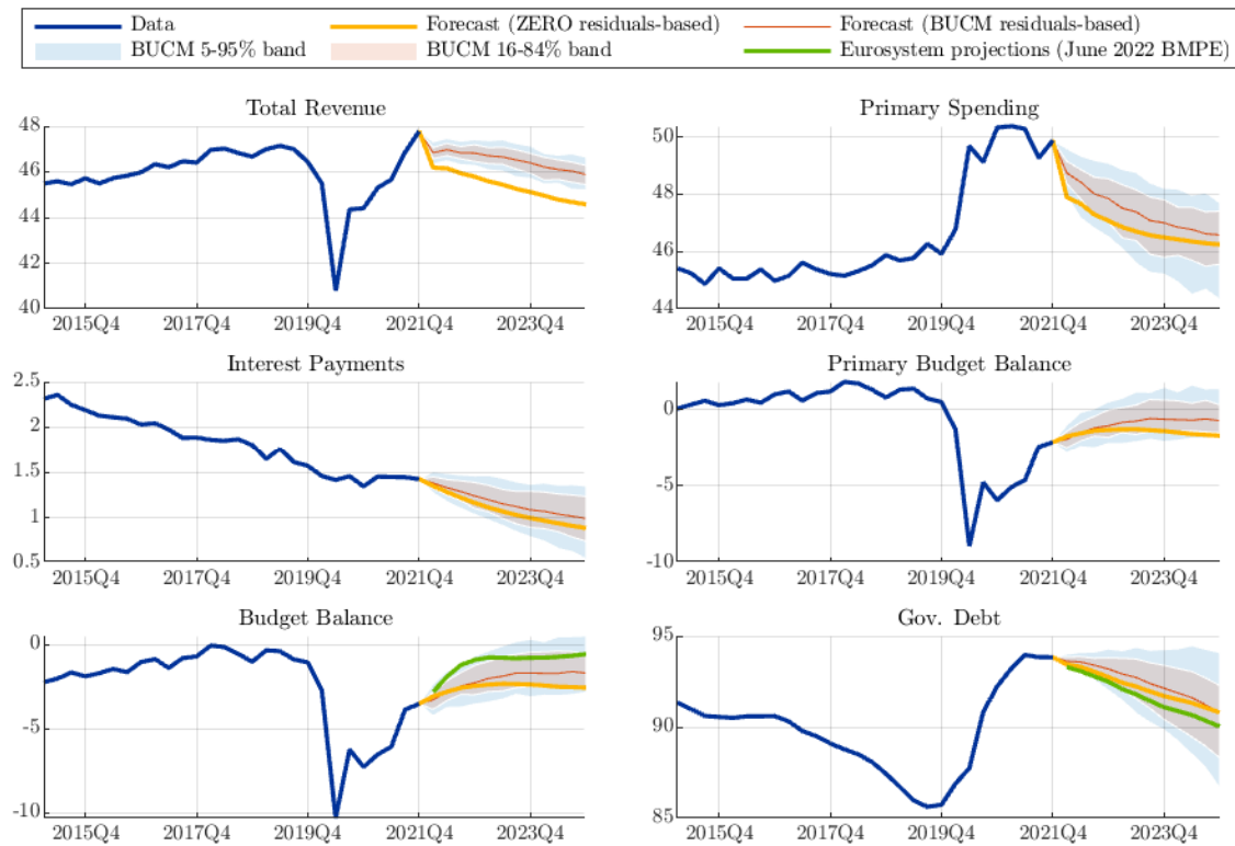
Figure 20: Stochastic projection of main fiscal variables (% of GDP)
