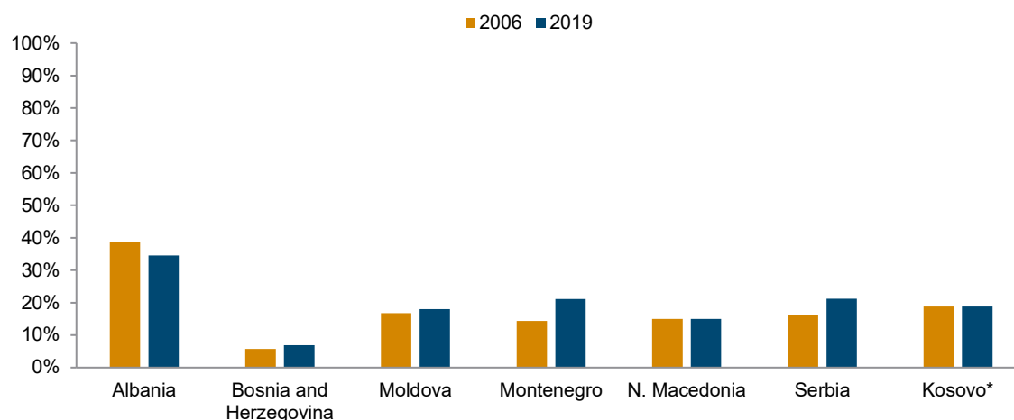
Figure 4 / Services imports as a percentage of total imports, 2006 and 2019
