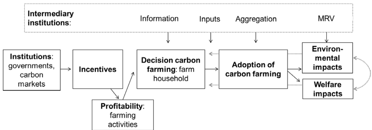
Figure 2. Conceptual framework
