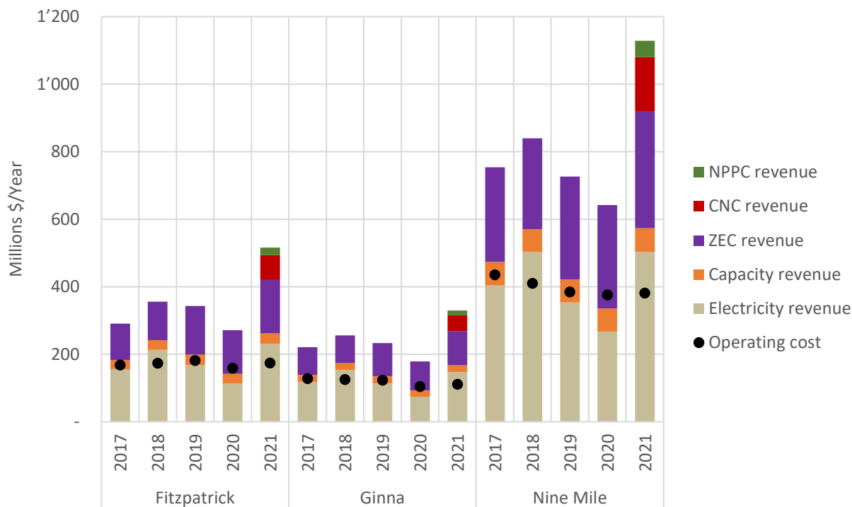
Figure 4. Profitability estimates of nuclear power plants in NYISO. Note: The black dot indicates estimated operating costs. Plants are earning money in a particular revenue scheme when the color for the scheme is higher than the black dot.
