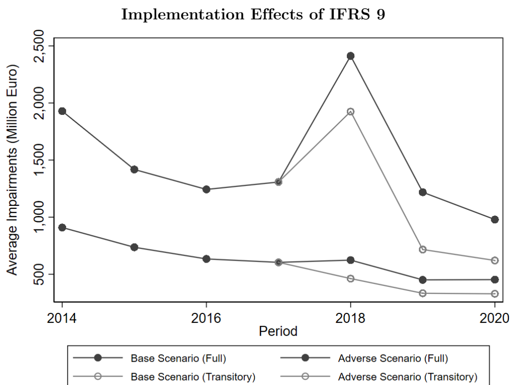
Figure 10: Comparison of the implementation effects in the baseline and adverse scenario.
