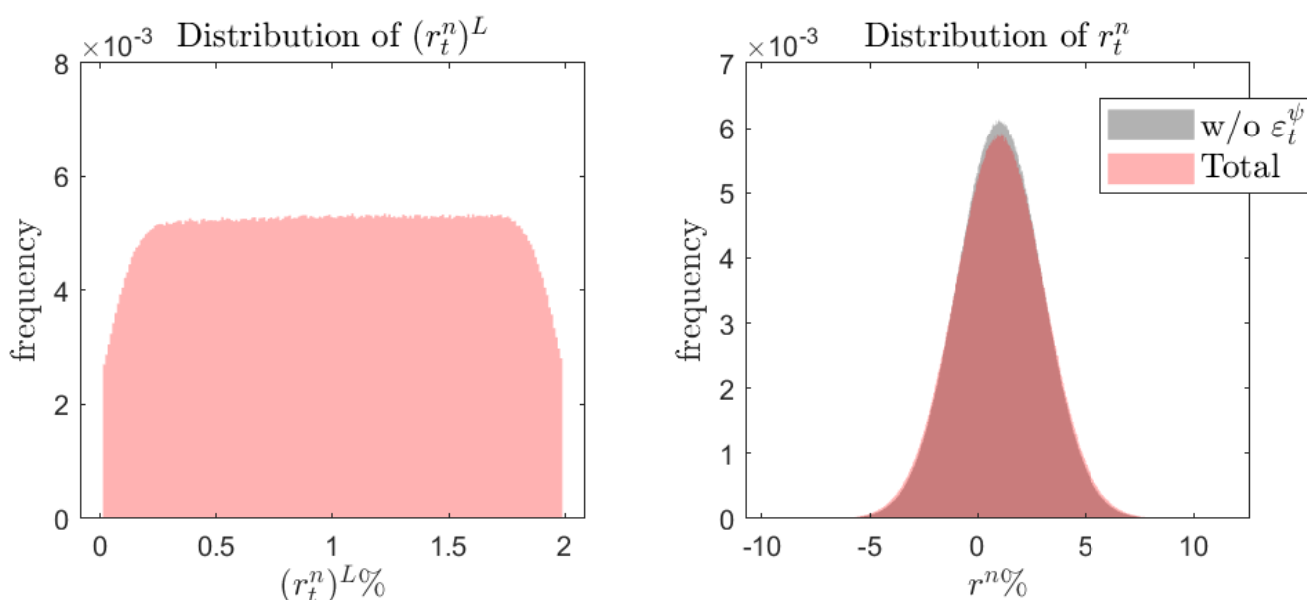
Figure 1: Unconditional distribution of the natural rate
